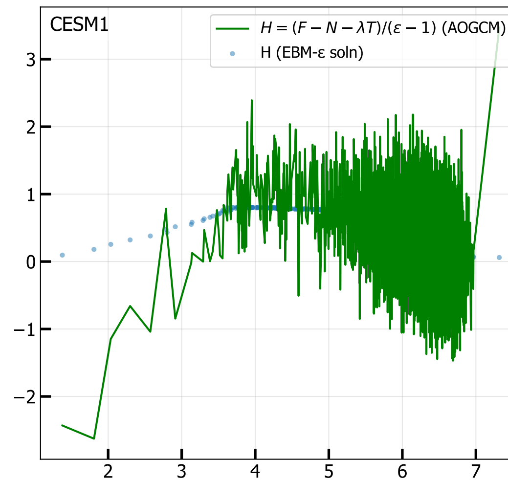
4xCO 2 Ocean Heat Uptake H vs T 2M (radiative fit, iter 3)
