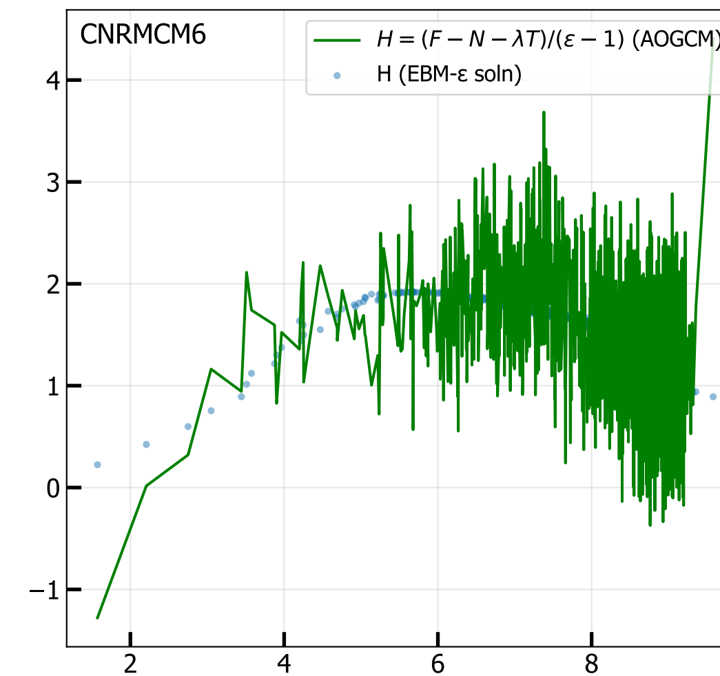
4xCO 2 Ocean Heat Uptake H vs T 2M (radiative fit, iter 4)
