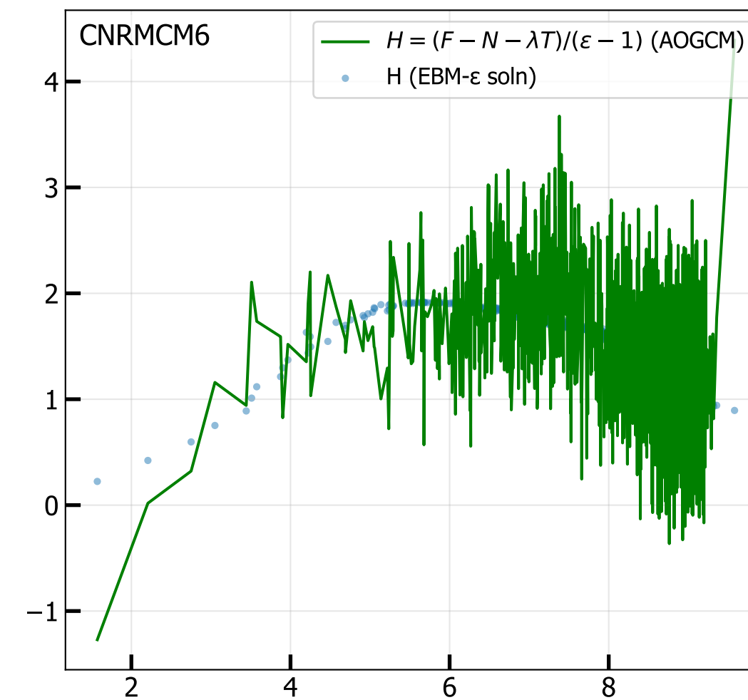
4xCO 2 Ocean Heat Uptake H vs T 2M (radiative fit, iter 7)
