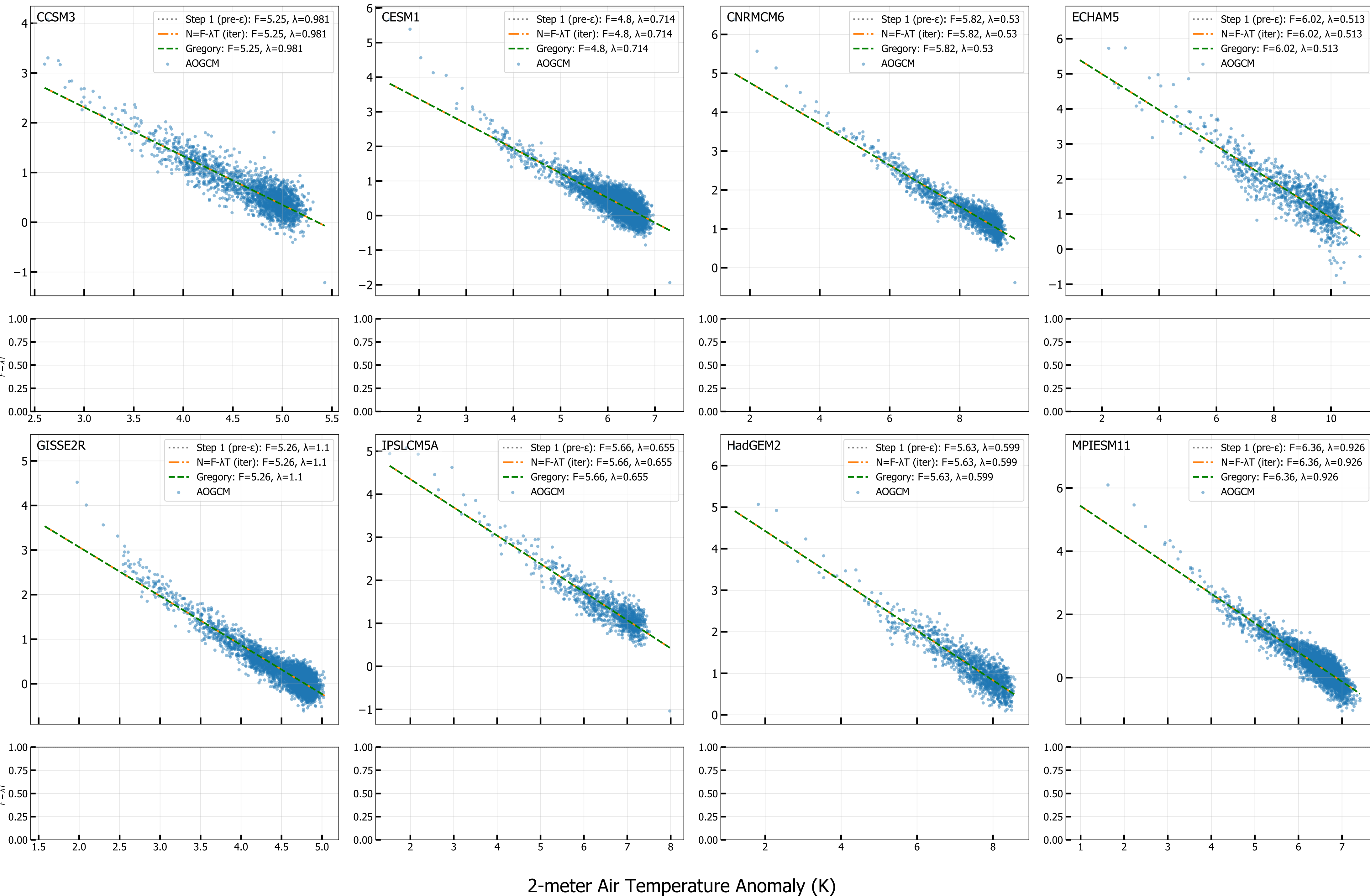
4xCO 2 Net TOA vs T 2M (radiative fit, iter 1)
