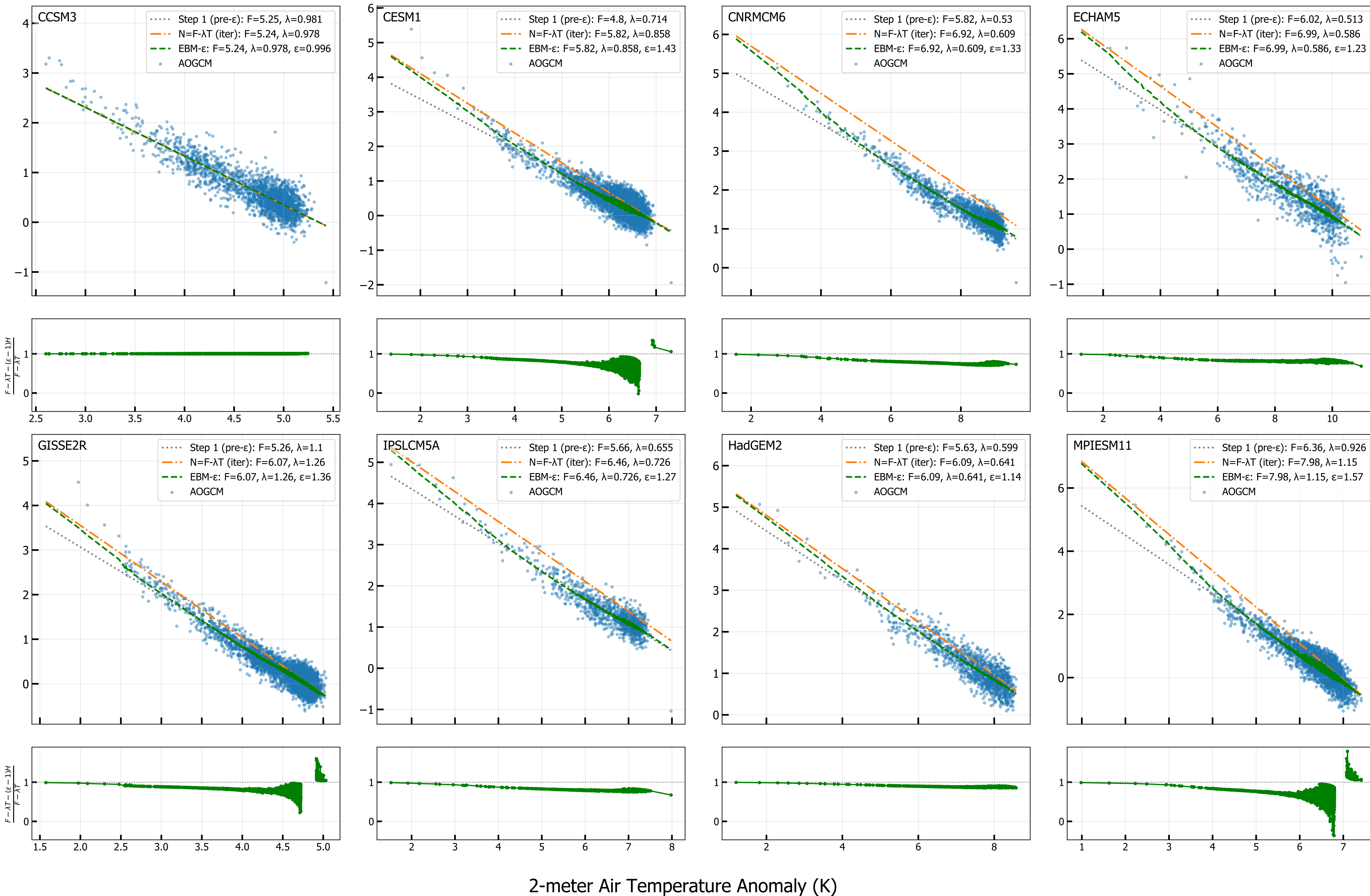
4xCO 2 Net TOA vs T 2M (radiative fit, iter 3)
