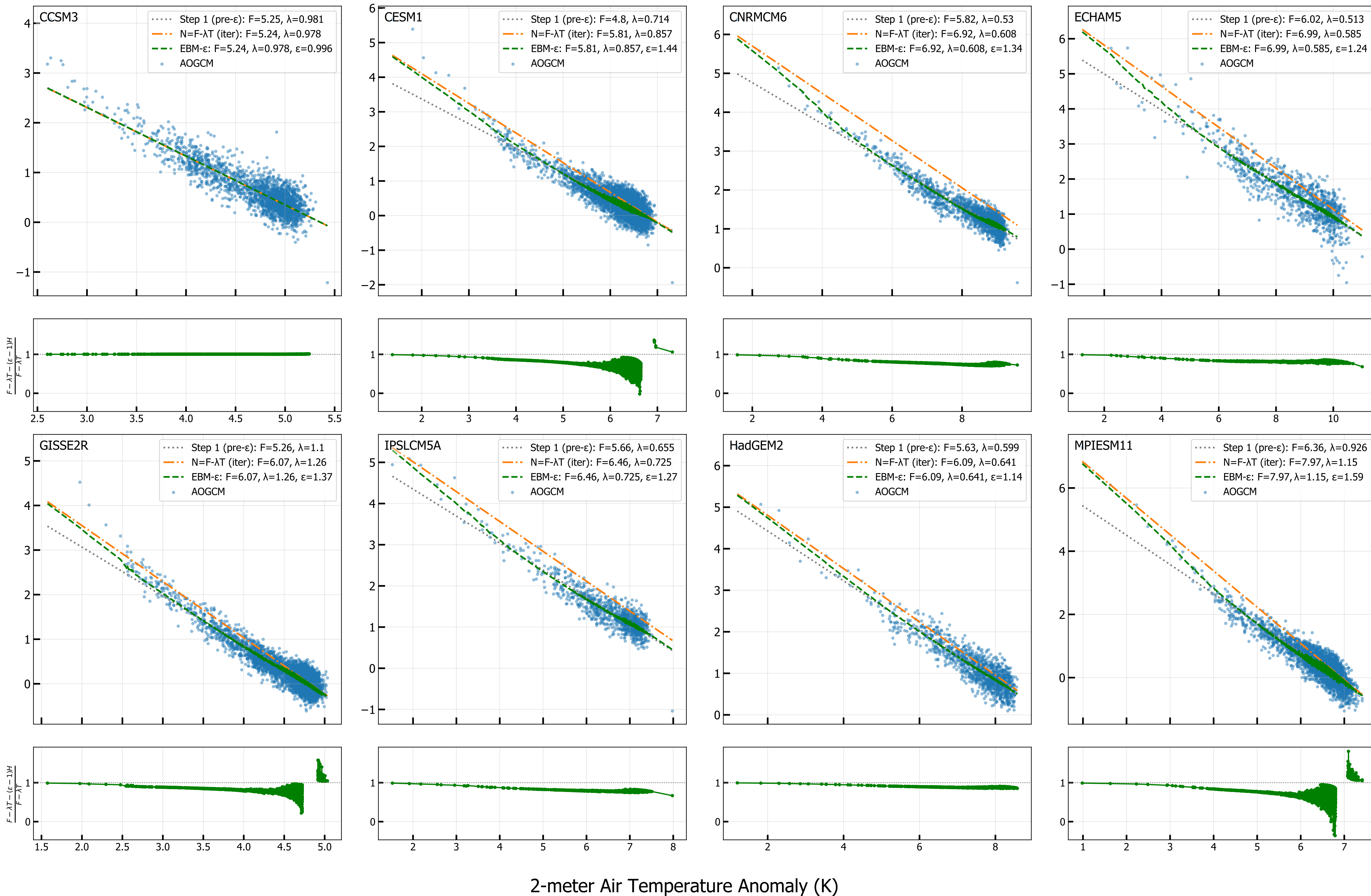
4xCO 2 Net TOA vs T 2M (radiative fit, iter 4)
