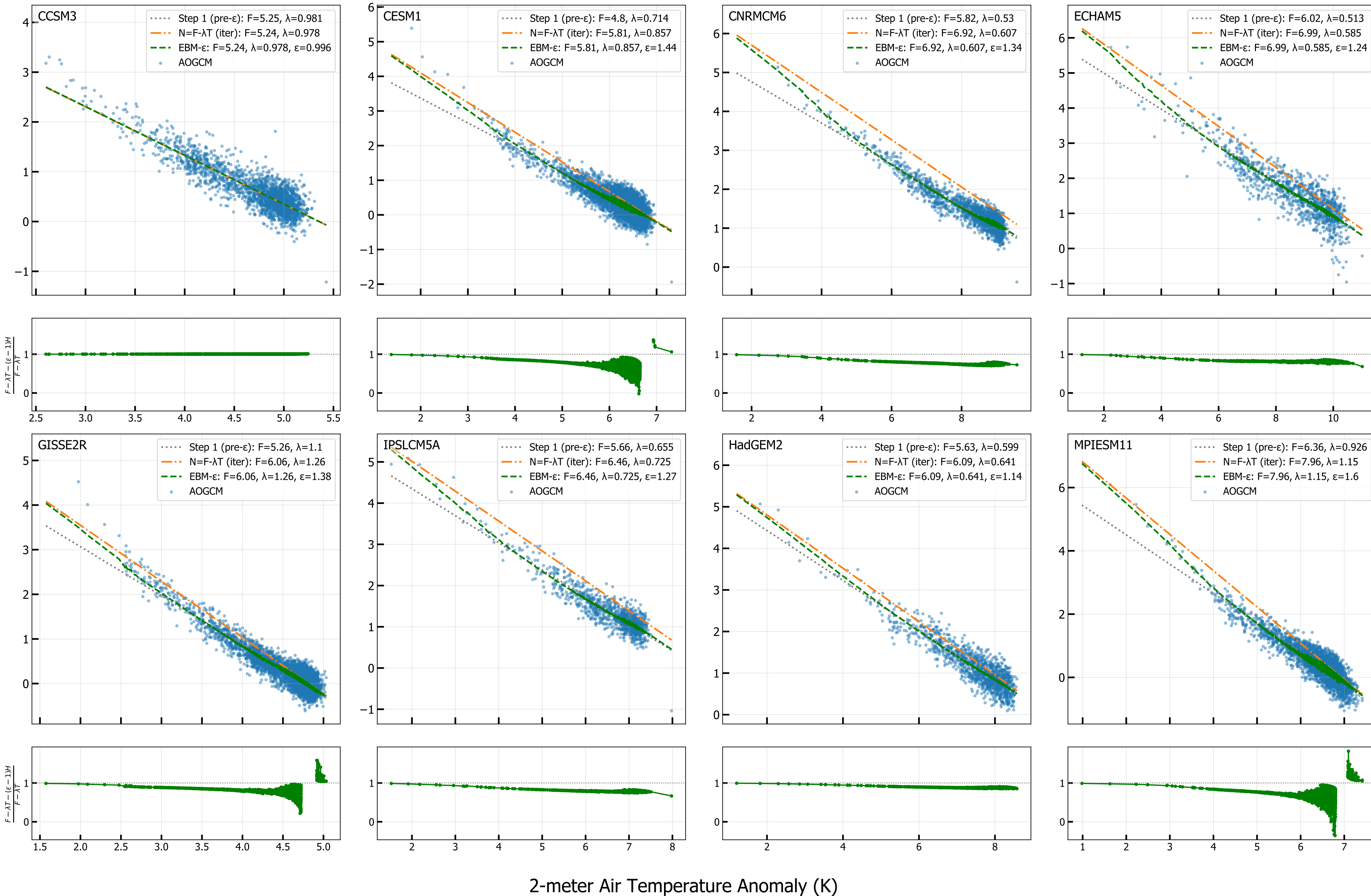
4xCO 2 Net TOA vs T 2M (radiative fit, iter 7)
