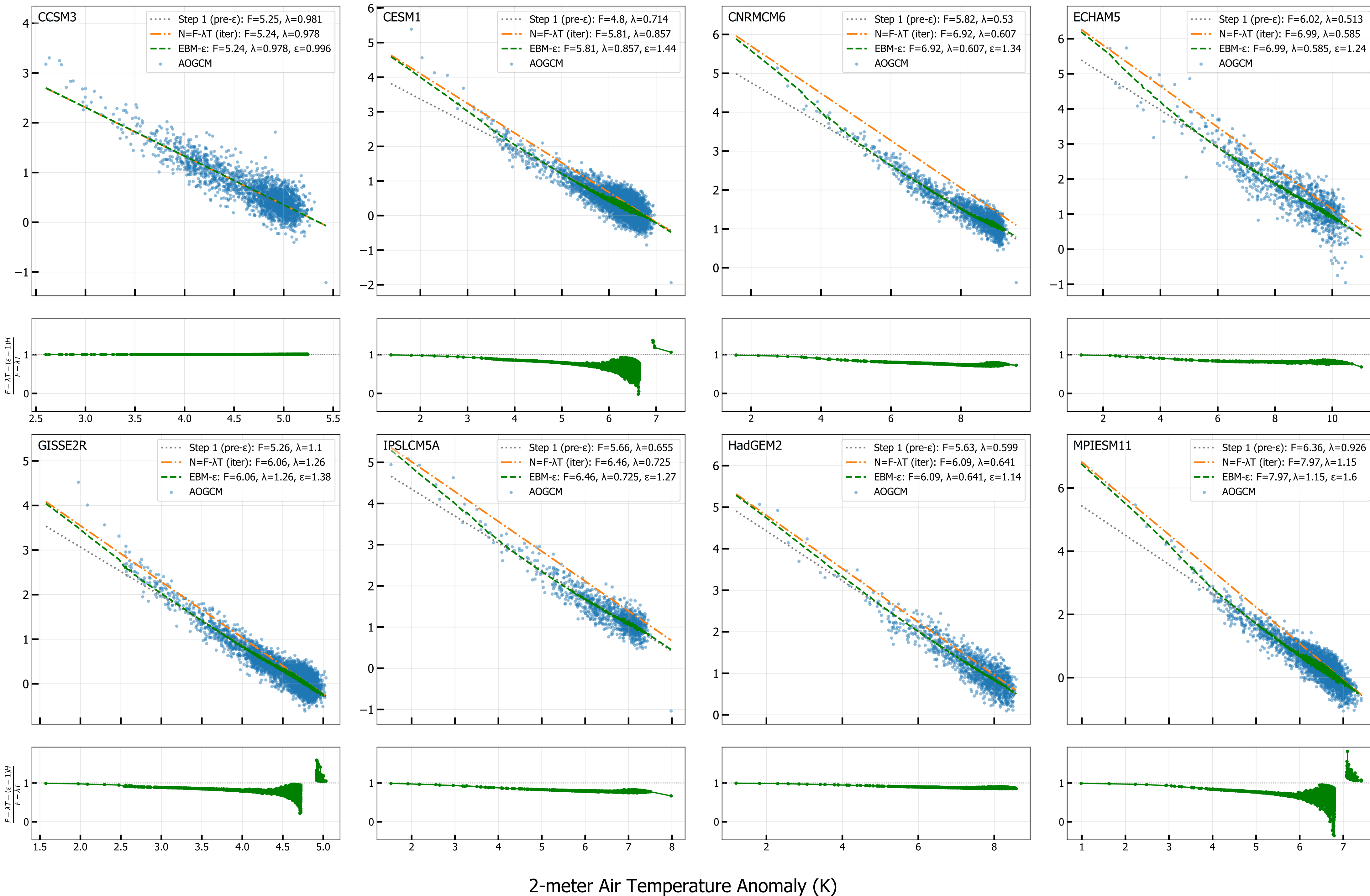
4xCO 2 Net TOA vs T 2M (radiative fit, iter 8)
