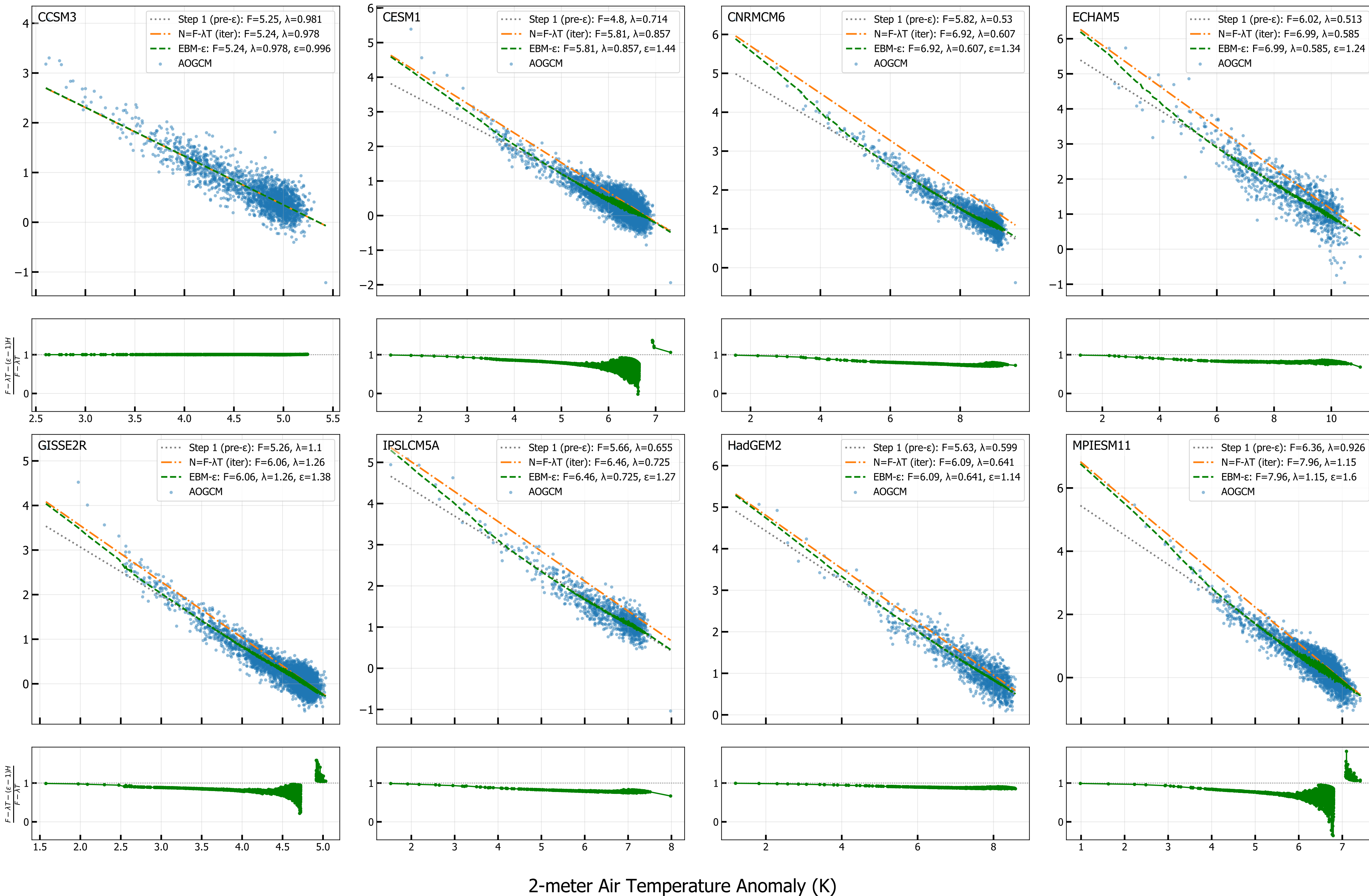
4xCO 2 Net TOA vs T 2M (radiative fit, iter 9)
