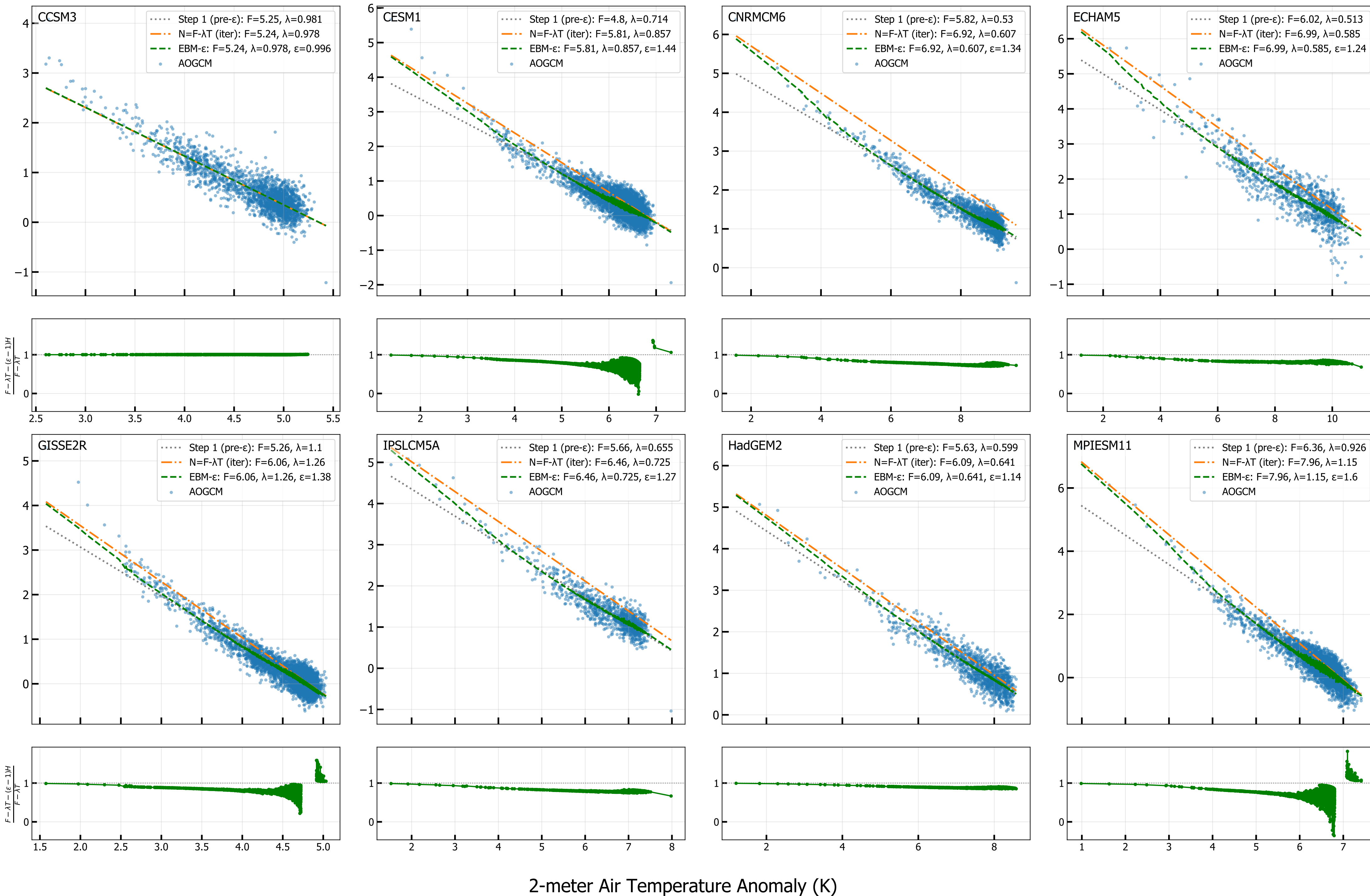
4xCO 2 Net TOA vs T 2M (radiative fit, iter 10)
