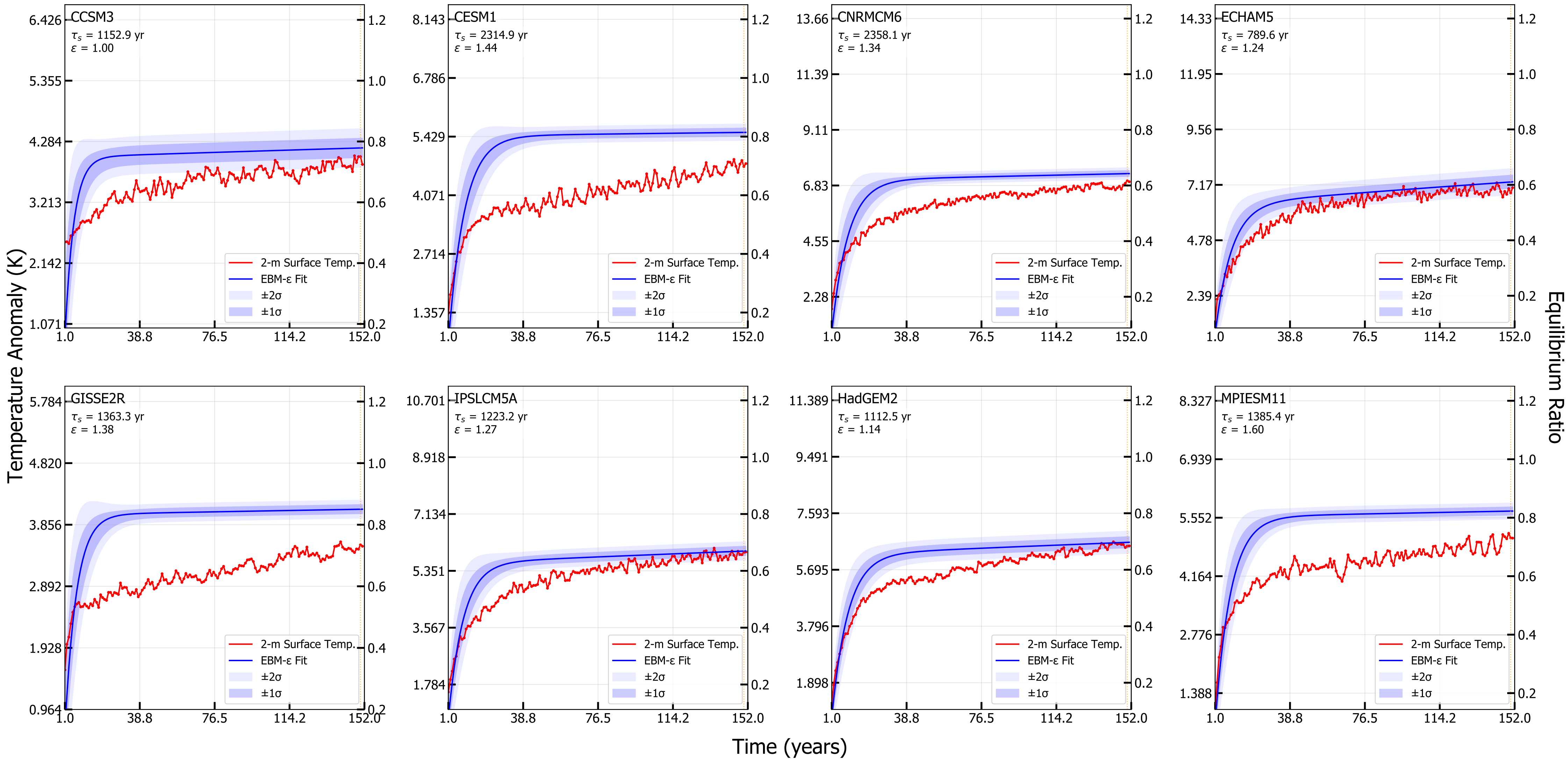
4xCO 2 T 2M vs. Time w/ EBM-ε Fit
