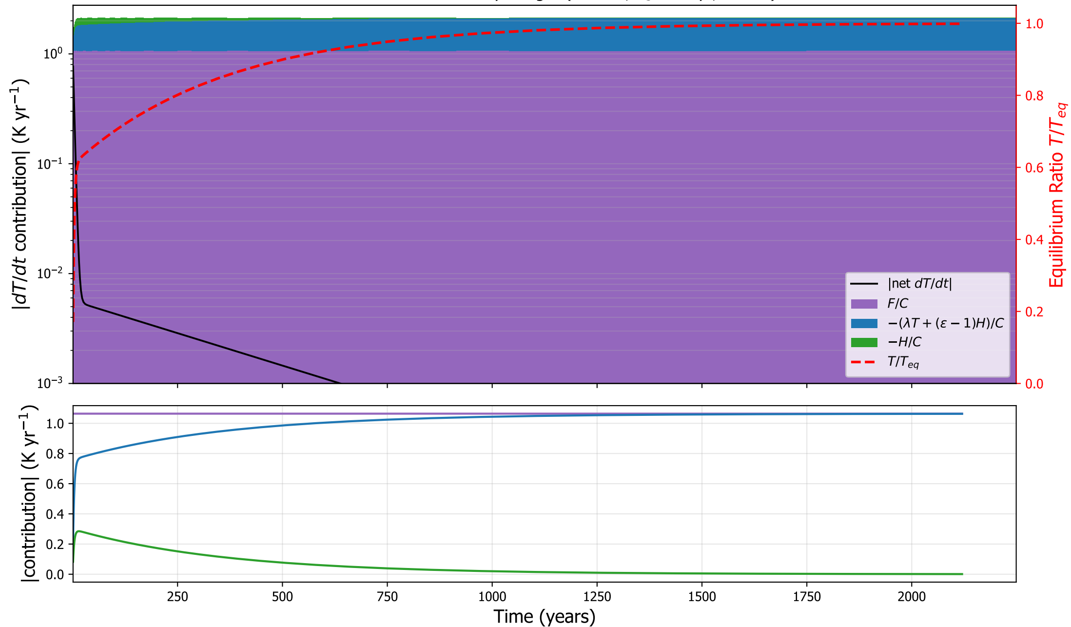
CCSM3: surface tendency budget ( \varepsilon=1.38 , \tau_s=368 yr, C=6.8 )
