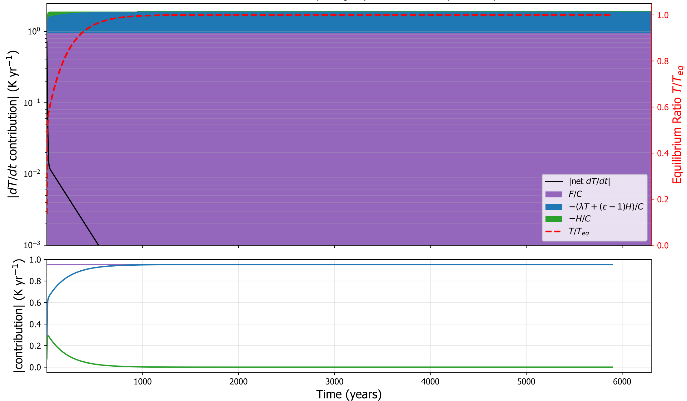
CESM1: surface tendency budget ( \varepsilon=1.35 , \tau_s=206 yr, C=8.0 )
