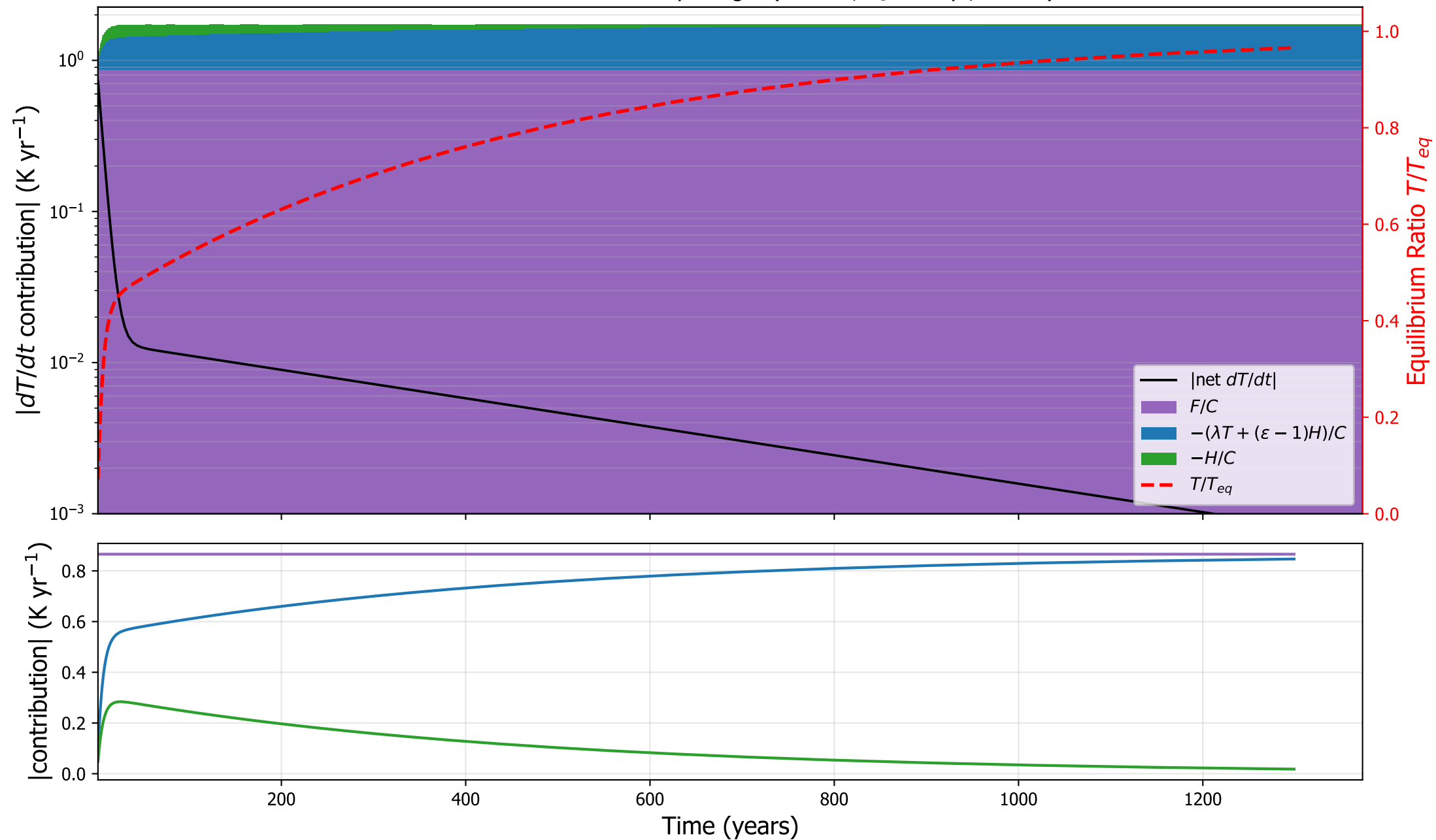
HadGEM2: surface tendency budget ( \varepsilon=1.58 , \tau_s=461 yr, C=7.9 )
