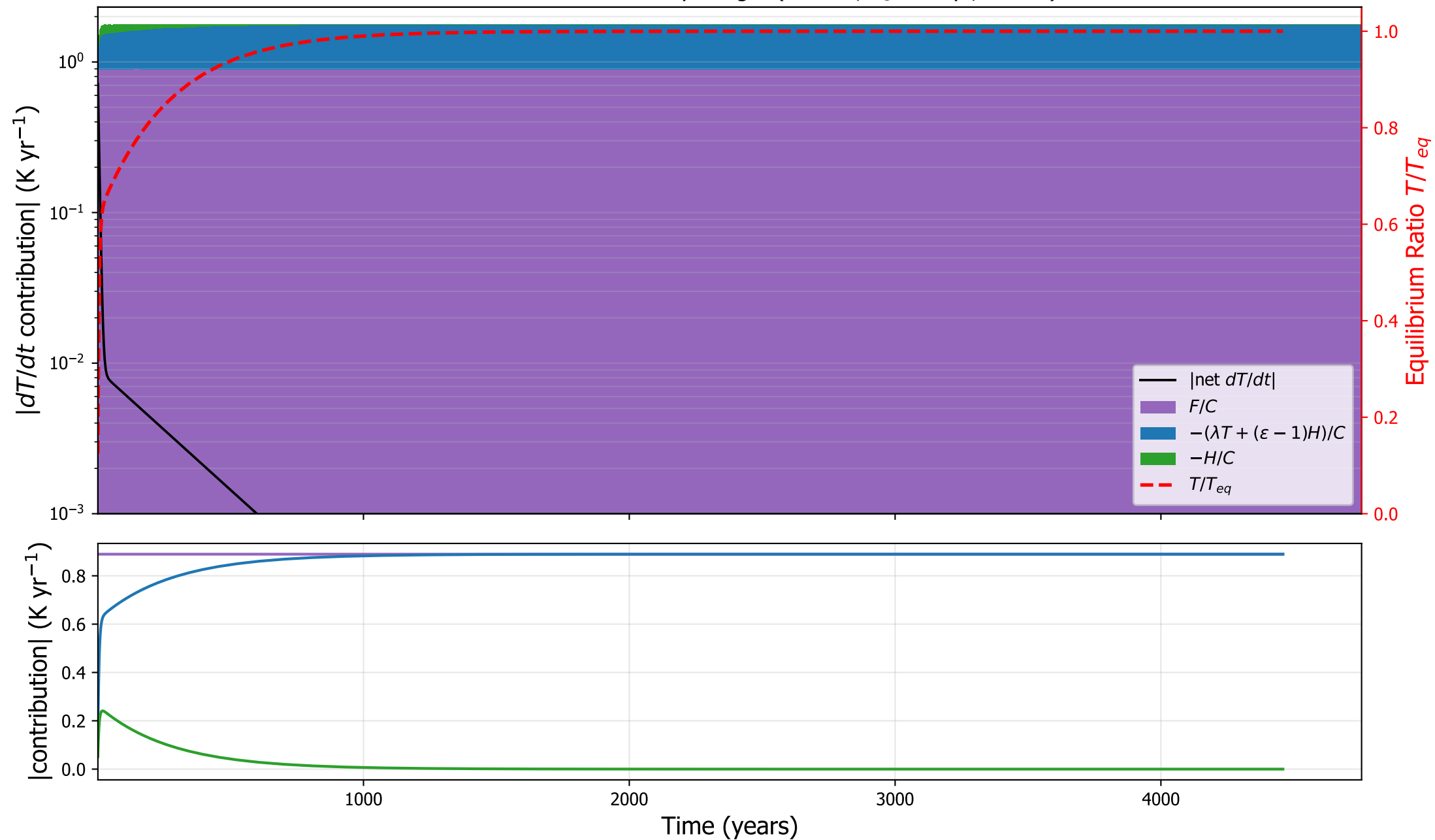
MPIESM11: surface tendency budget ( \varepsilon=1.27 , \tau_s=272 yr, C=9.9 )
