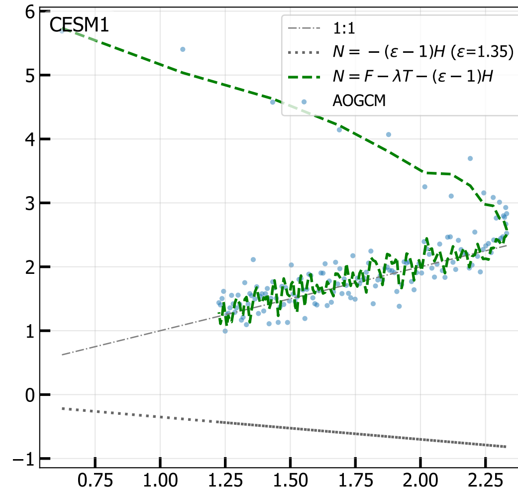
4xCO 2 Net TOA vs Ocean Heat Uptake H (radiative fit, iter 6)
