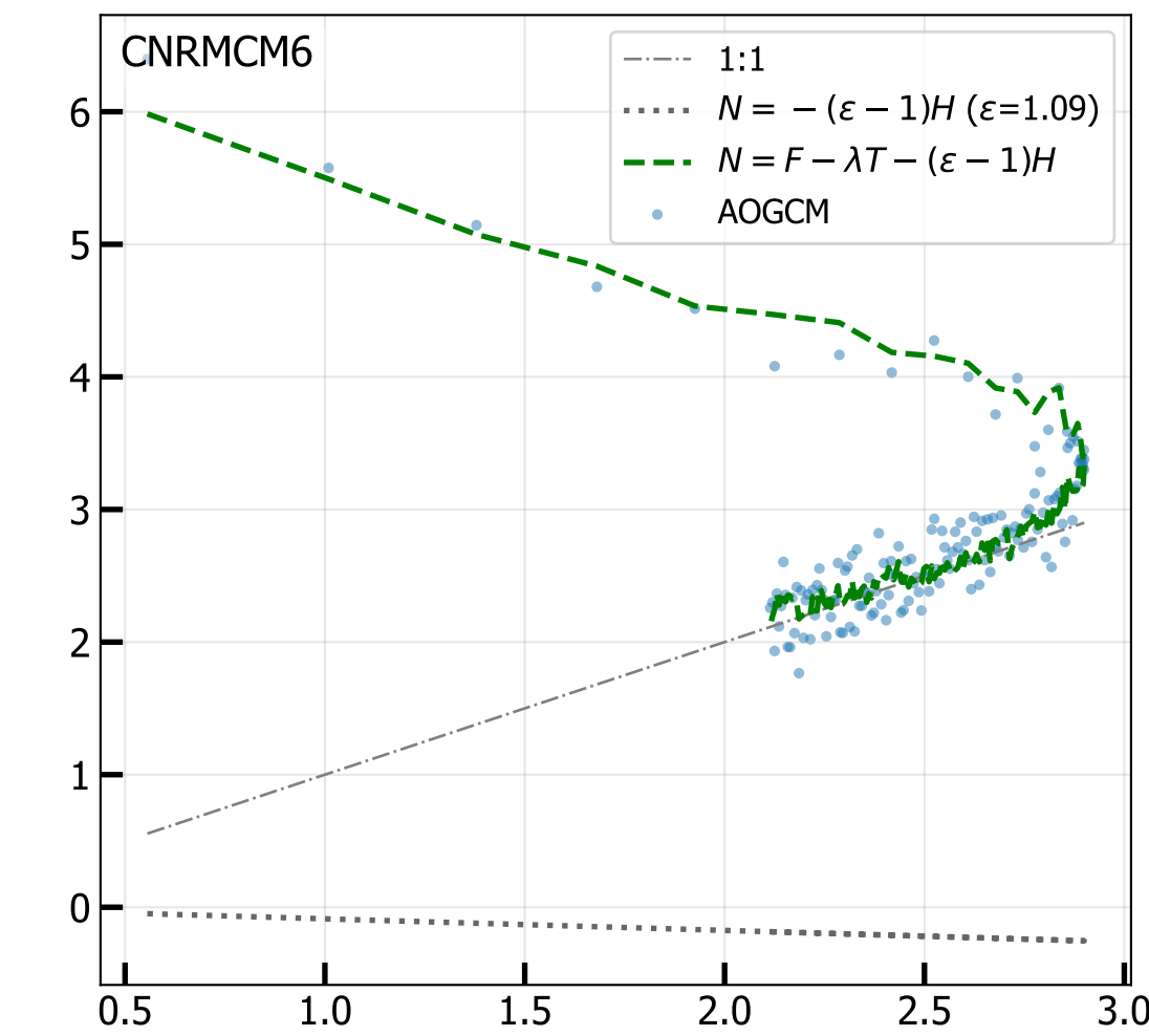
4xCO 2 Net TOA vs Ocean Heat Uptake H (radiative fit, iter 6)
