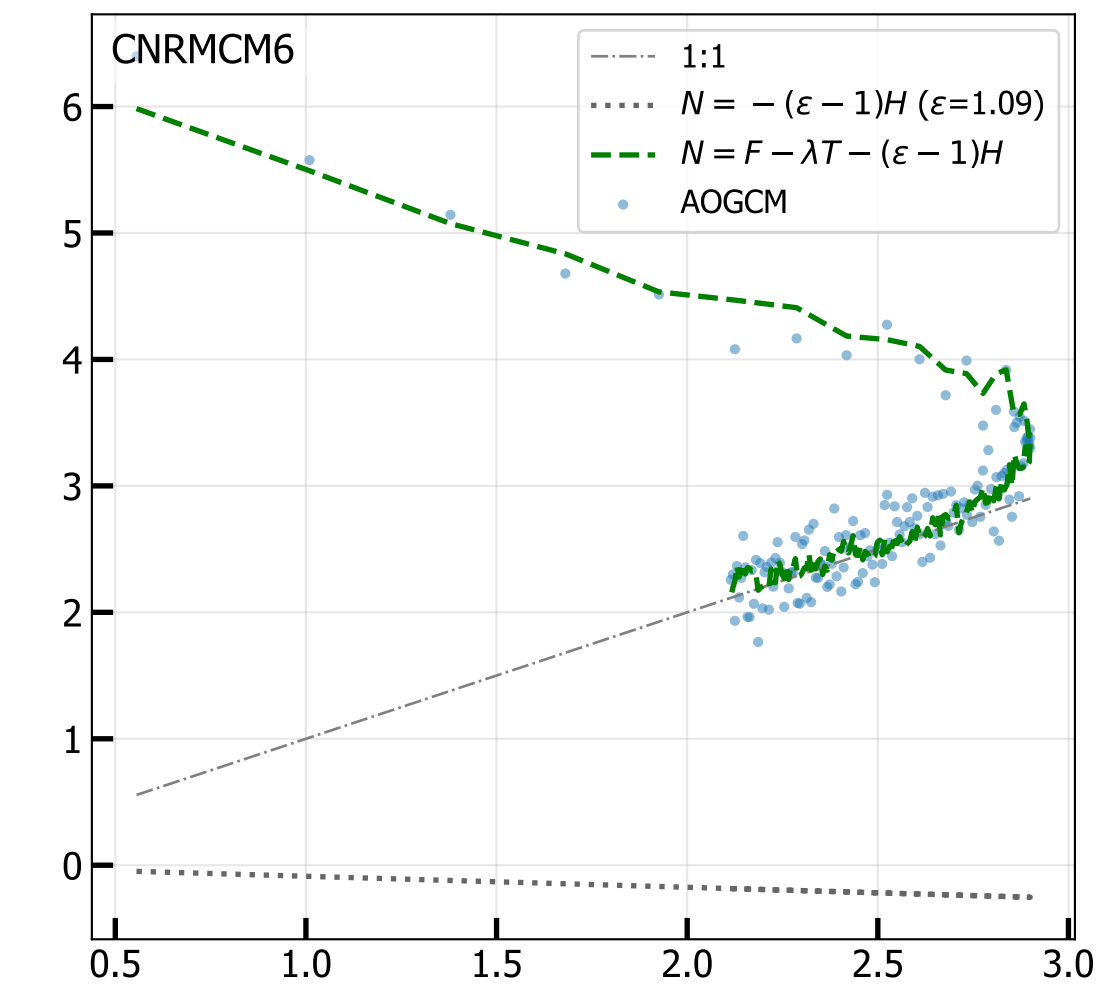
4xCO 2 Net TOA vs Ocean Heat Uptake H (radiative fit, iter 7)
