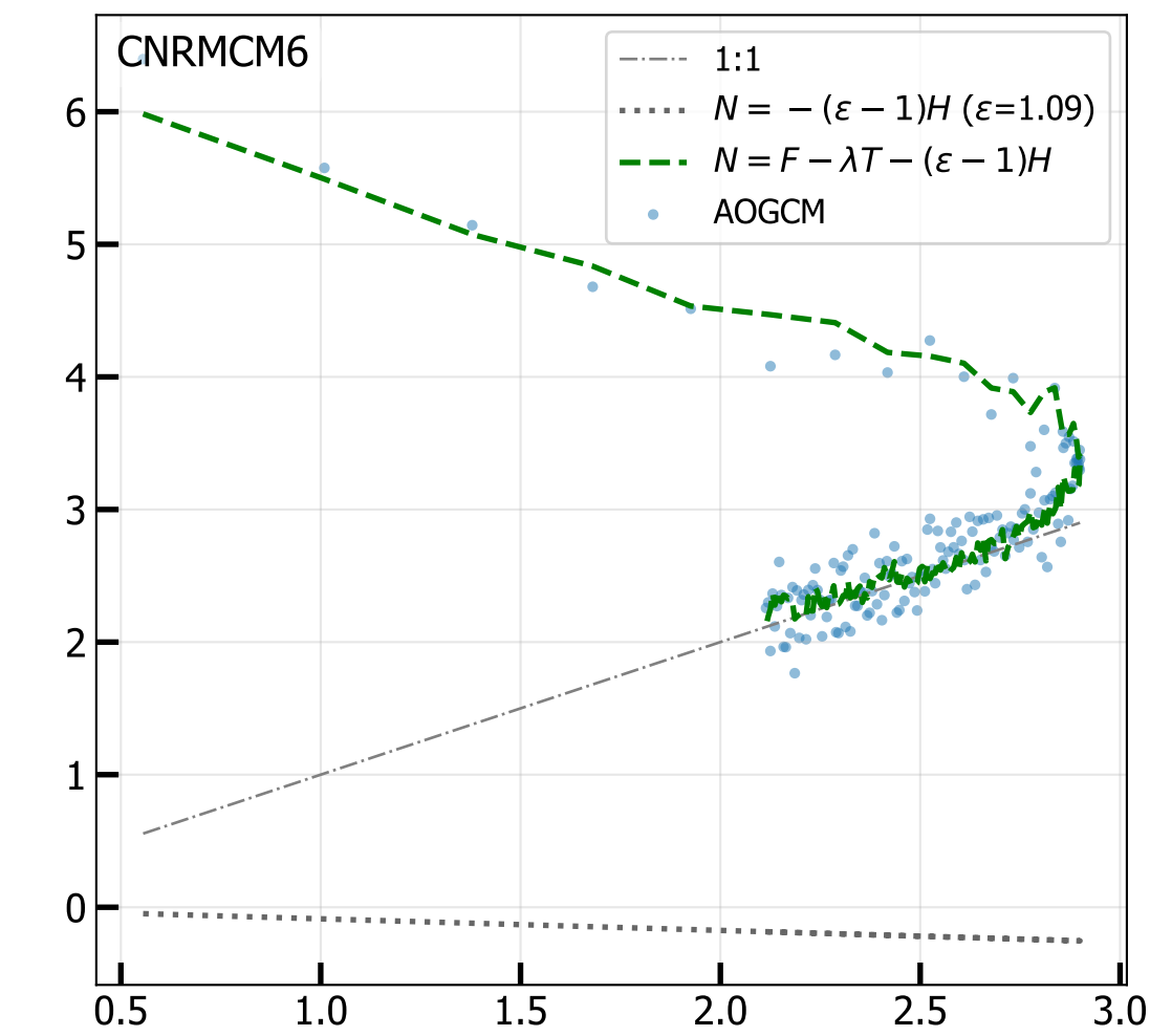
4xCO 2 Net TOA vs Ocean Heat Uptake H (radiative fit, iter 9)
