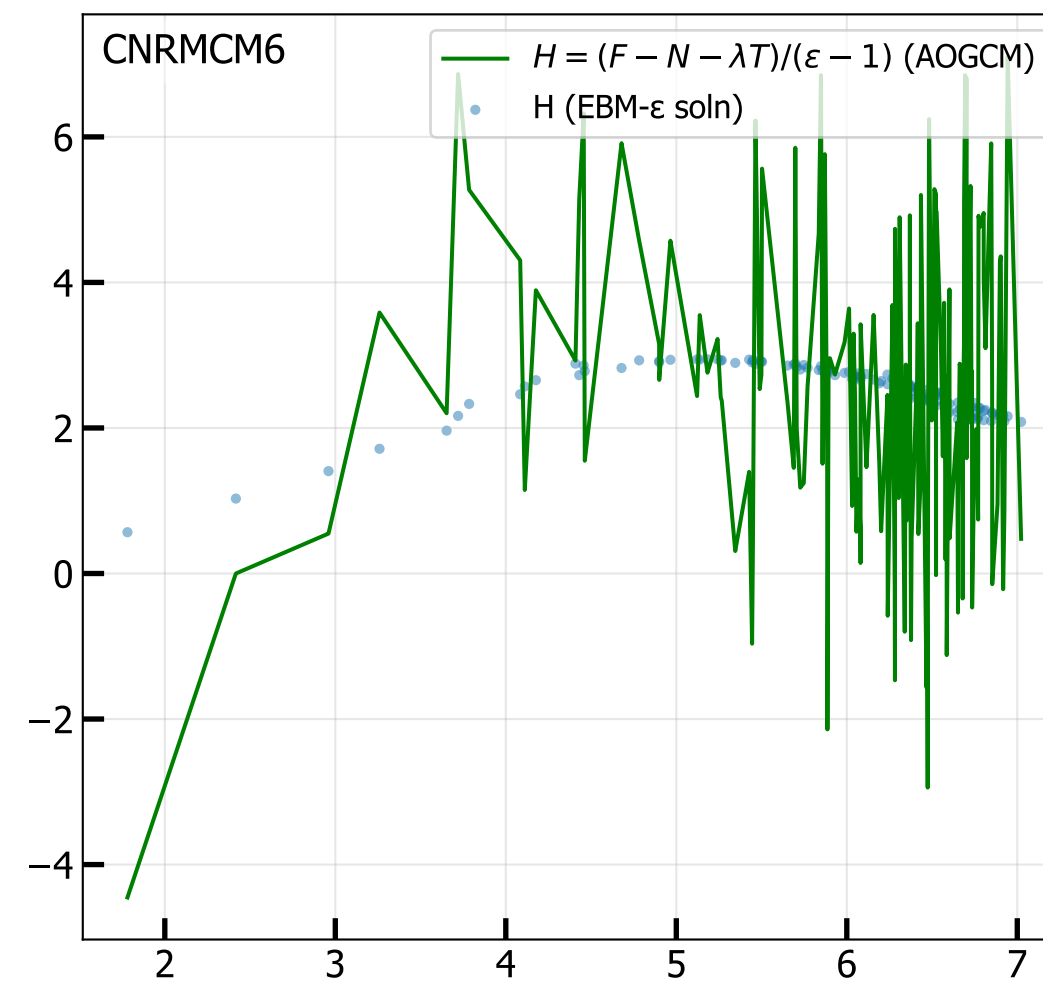
4xCO 2 Ocean Heat Uptake H vs T 2M (radiative fit, iter 2)
