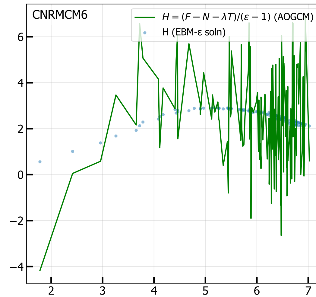
4xCO 2 Ocean Heat Uptake H vs T 2M (radiative fit, iter 6)
