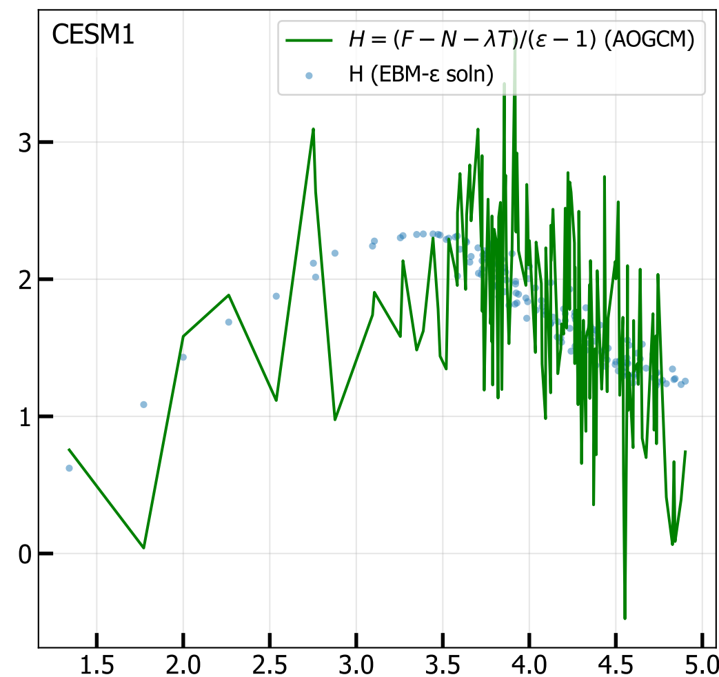
4xCO 2 Ocean Heat Uptake H vs T 2M (radiative fit, iter 8)
