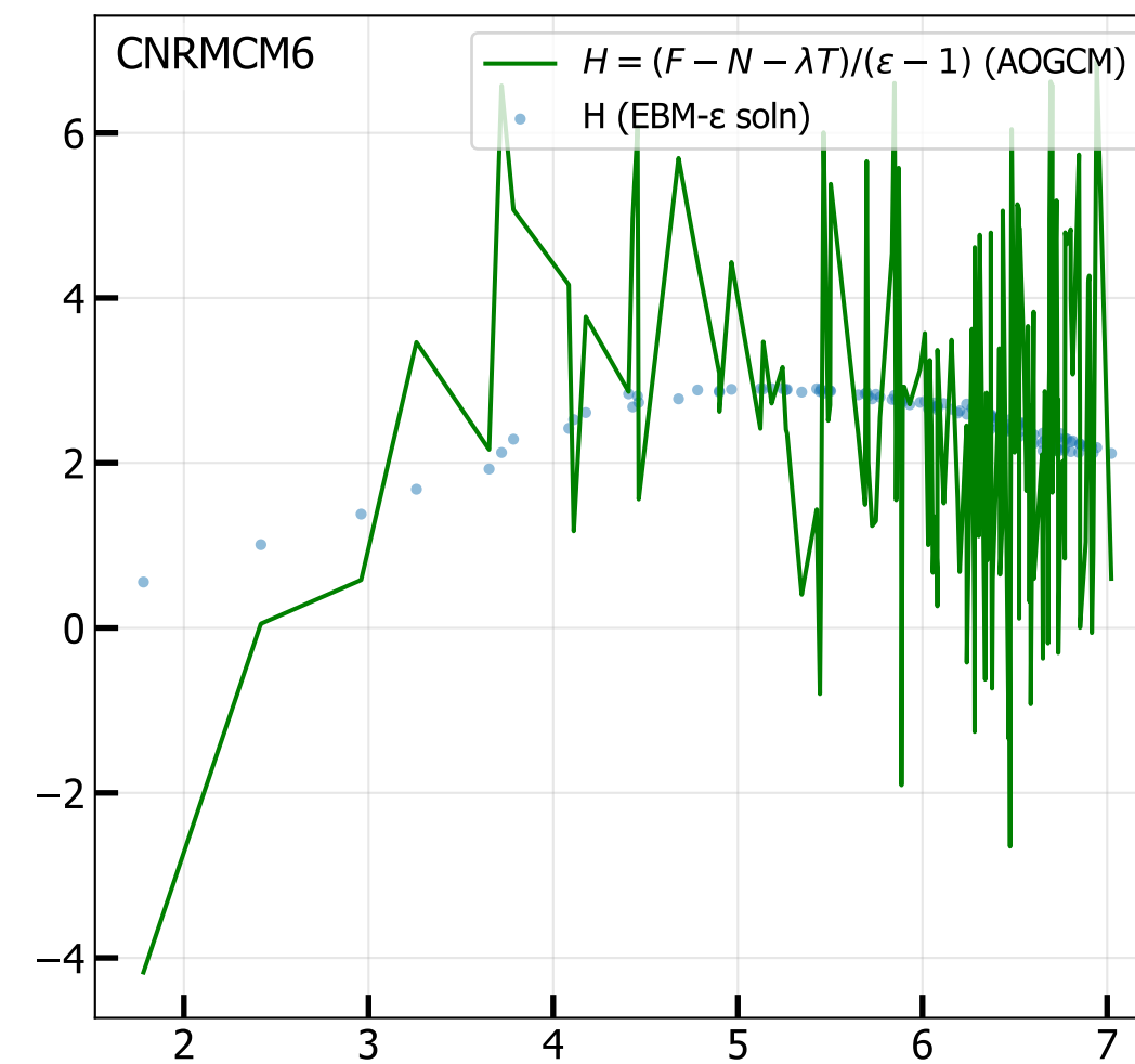
4xCO 2 Ocean Heat Uptake H vs T 2M (radiative fit, iter 9)
