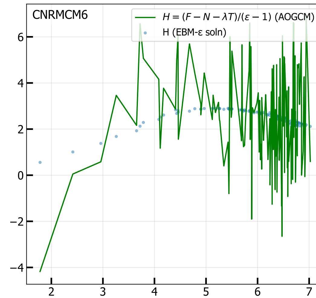
4xCO 2 Ocean Heat Uptake H vs T 2M (radiative fit, iter 10)
