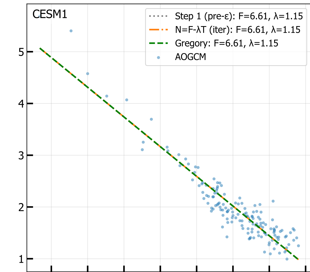
4xCO 2 Net TOA vs T 2M (radiative fit, iter 1)
