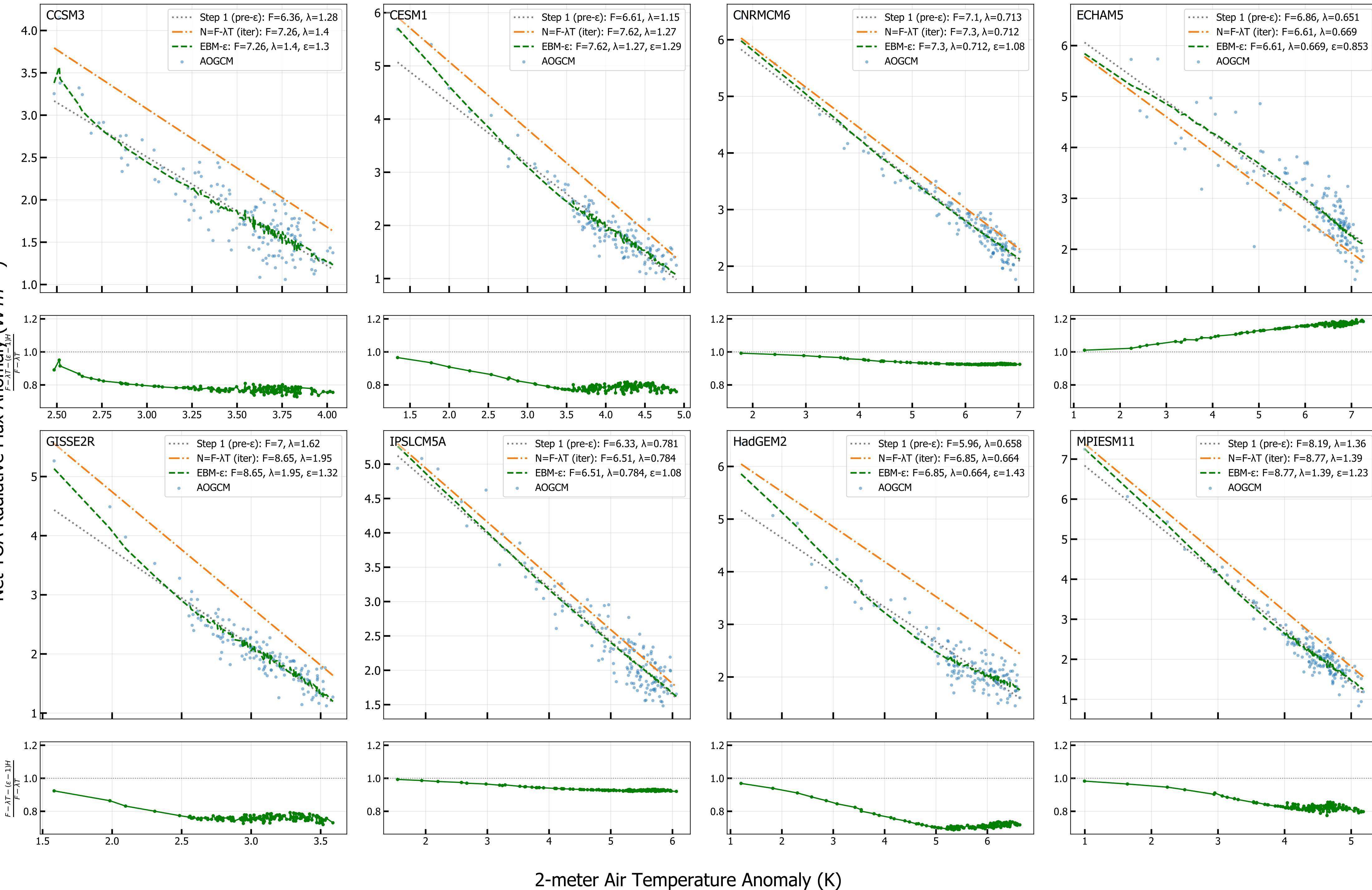
4xCO 2 Net TOA vs T 2M (radiative fit, iter 2)
