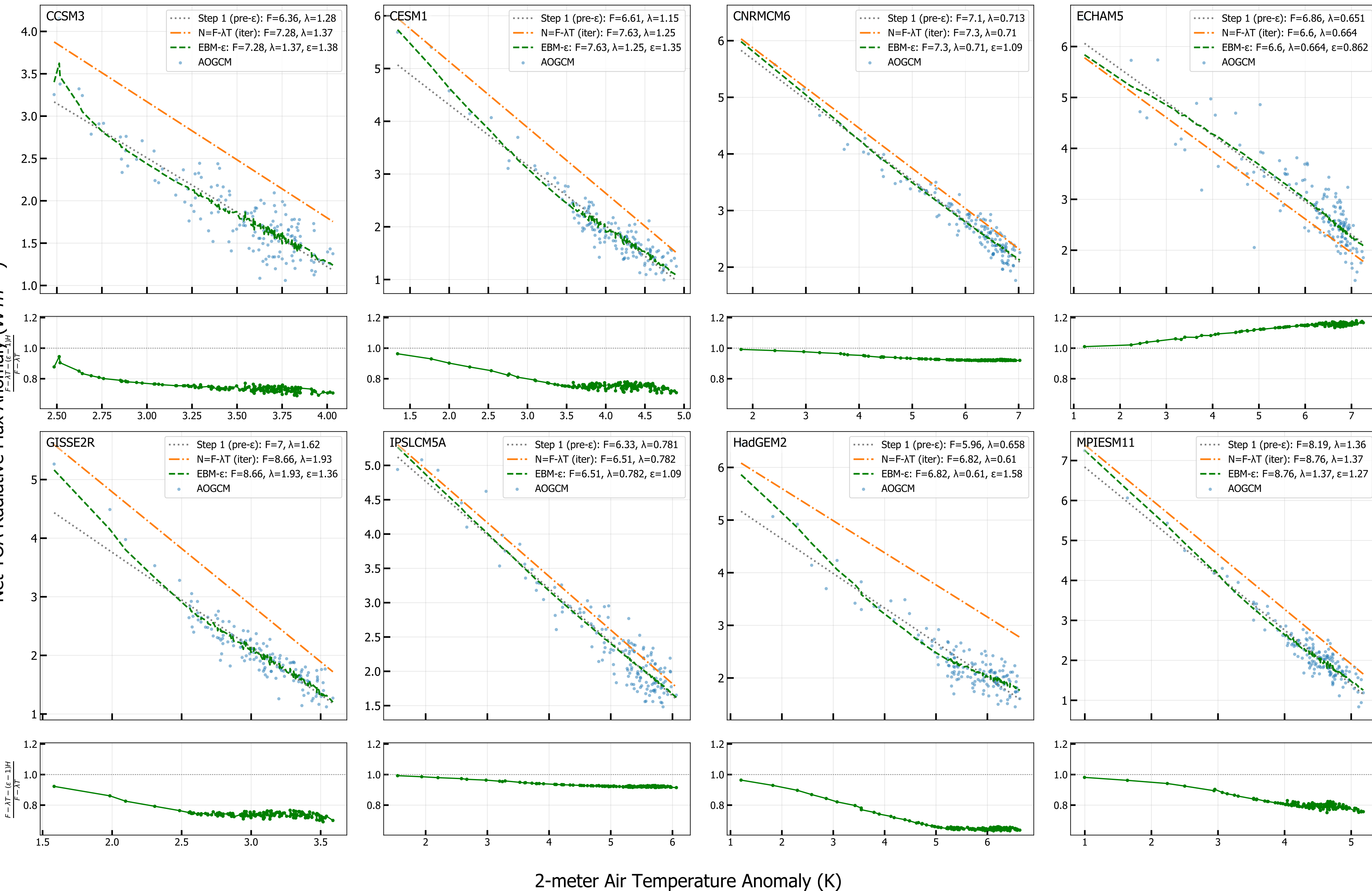
4xCO 2 Net TOA vs T 2M (radiative fit, iter 6)
