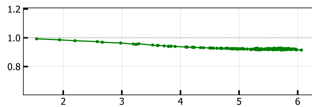
2-meter Air Temperature Anomaly (K)
