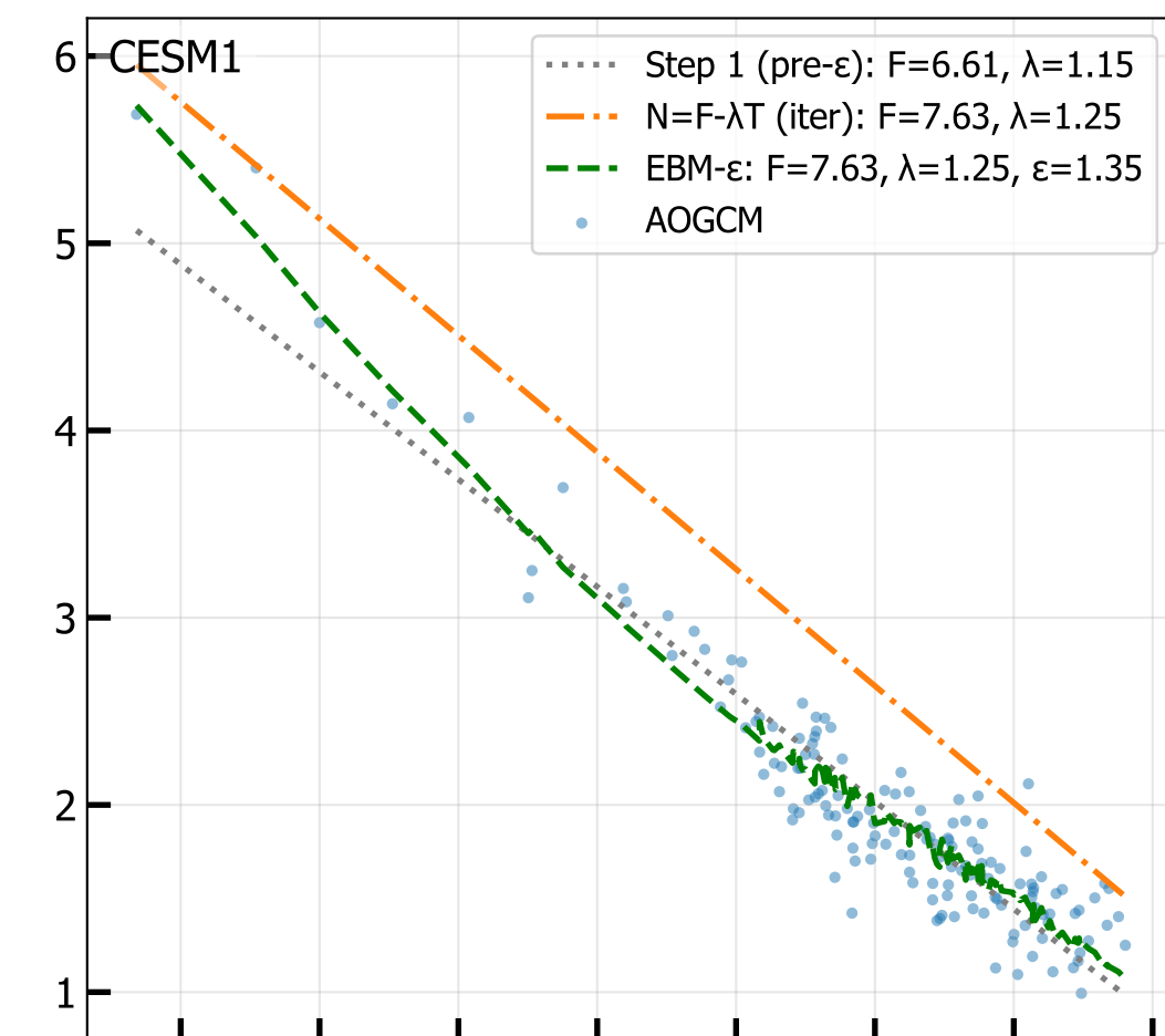
4xCO 2 Net TOA vs T 2M (radiative fit, iter 7)
