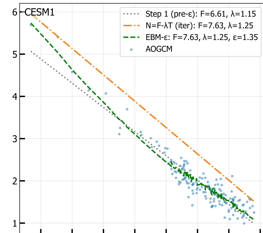
4xCO 2 Net TOA vs T 2M (radiative fit, iter 8)
