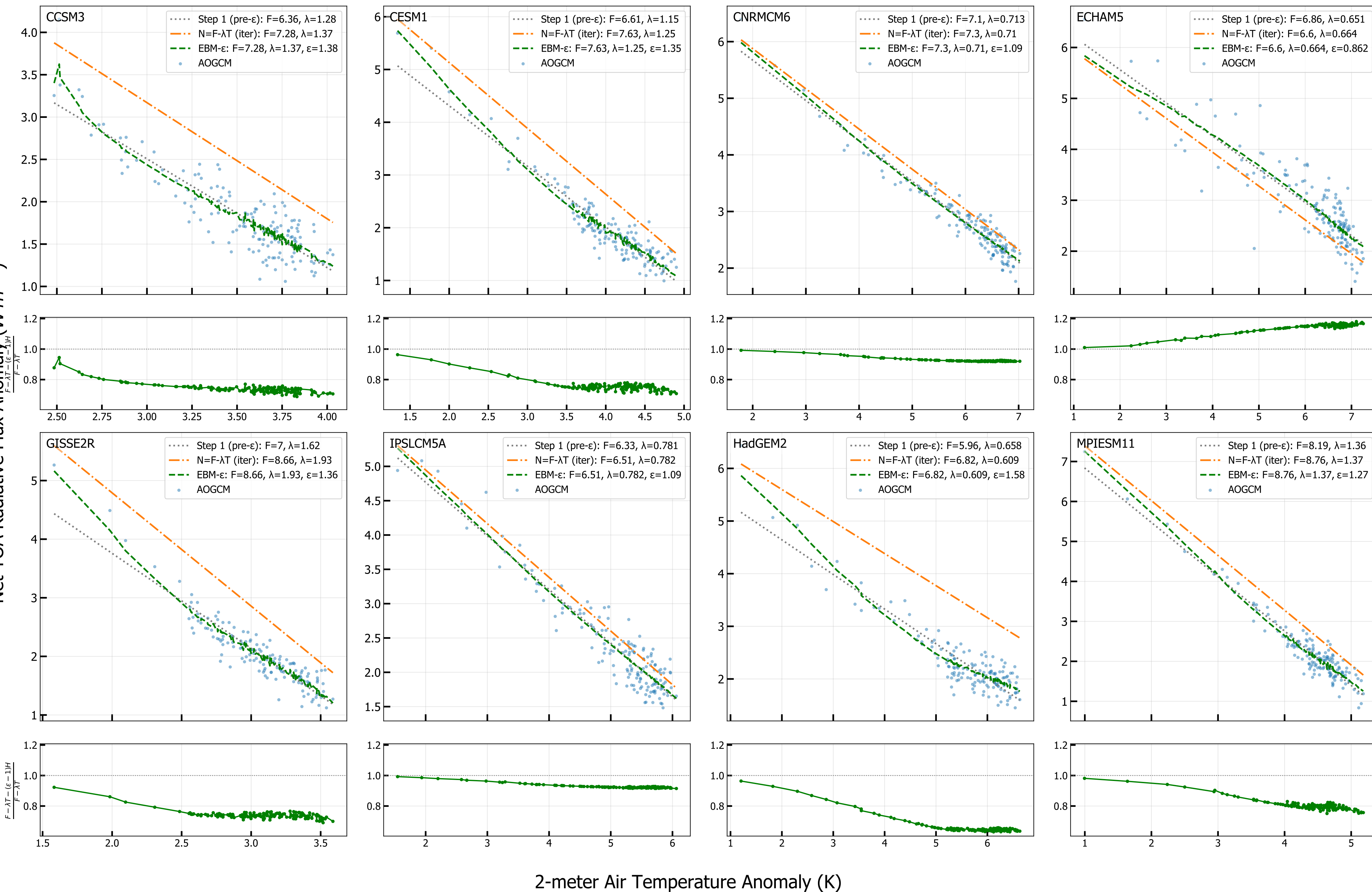
4xCO 2 Net TOA vs T 2M (radiative fit, iter 10)
