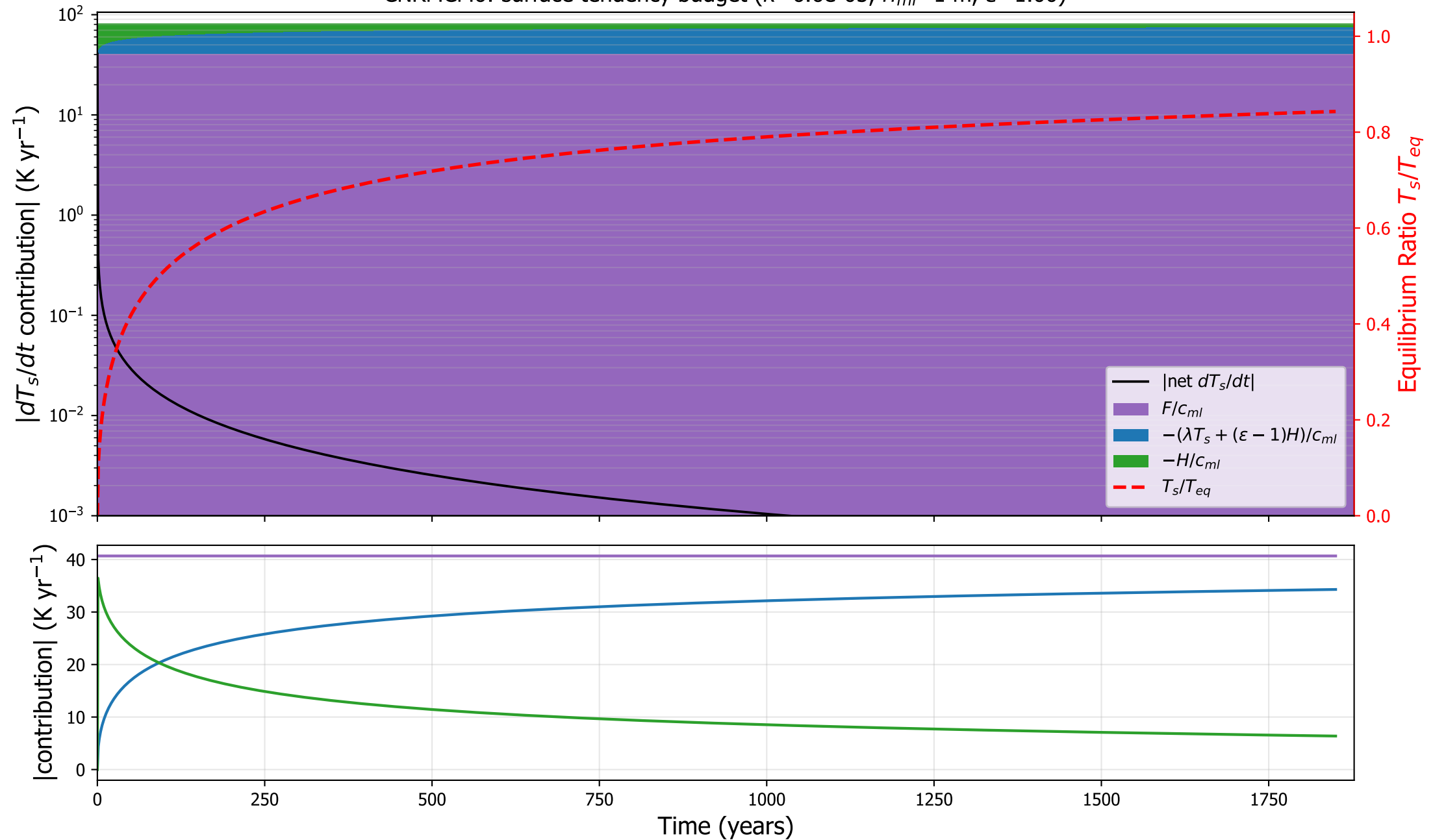
CNRMCM6: surface tendency budget ( \kappa=6.6\text{e-}05 , h_{ml}=1 m, \varepsilon=1.00 )
