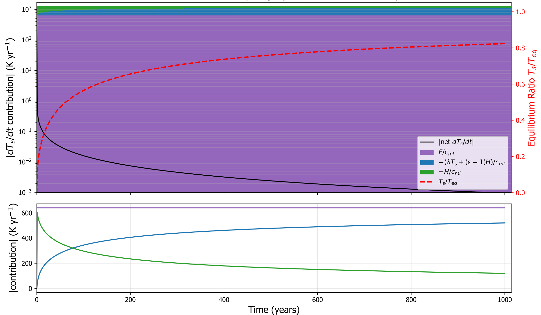
ECHAM5: surface tendency budget ( \kappa=4.2\text{e-}05 , h_{ml}=0 m, \varepsilon=0.94 )
