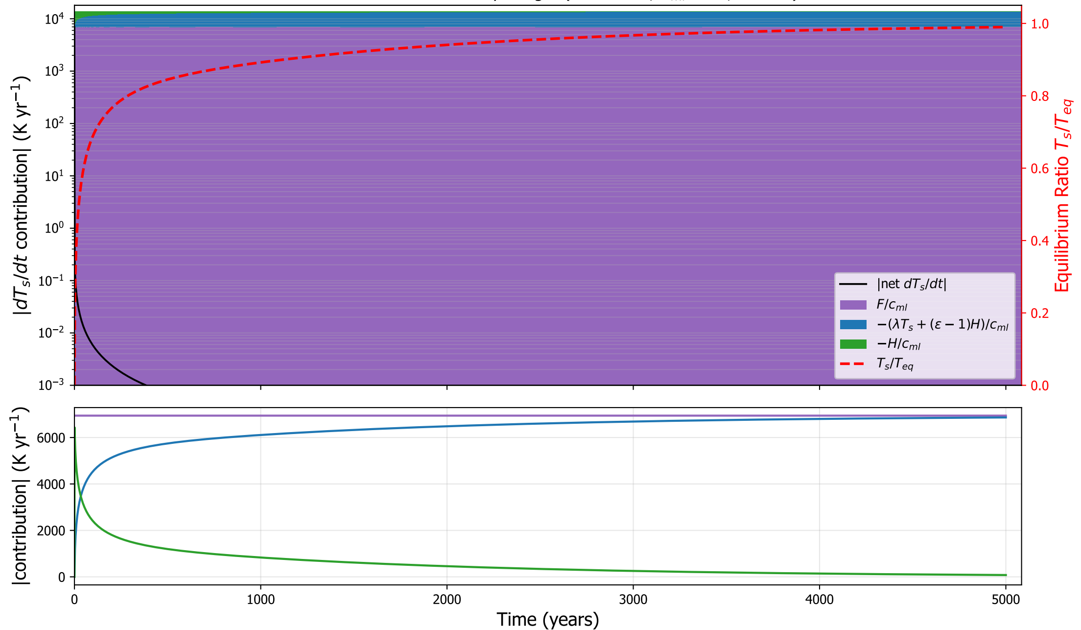
GISSE2R: surface tendency budget ( \kappa=1.5\text{e-}04 , h_{ml}=0 m, \varepsilon=0.90 )
