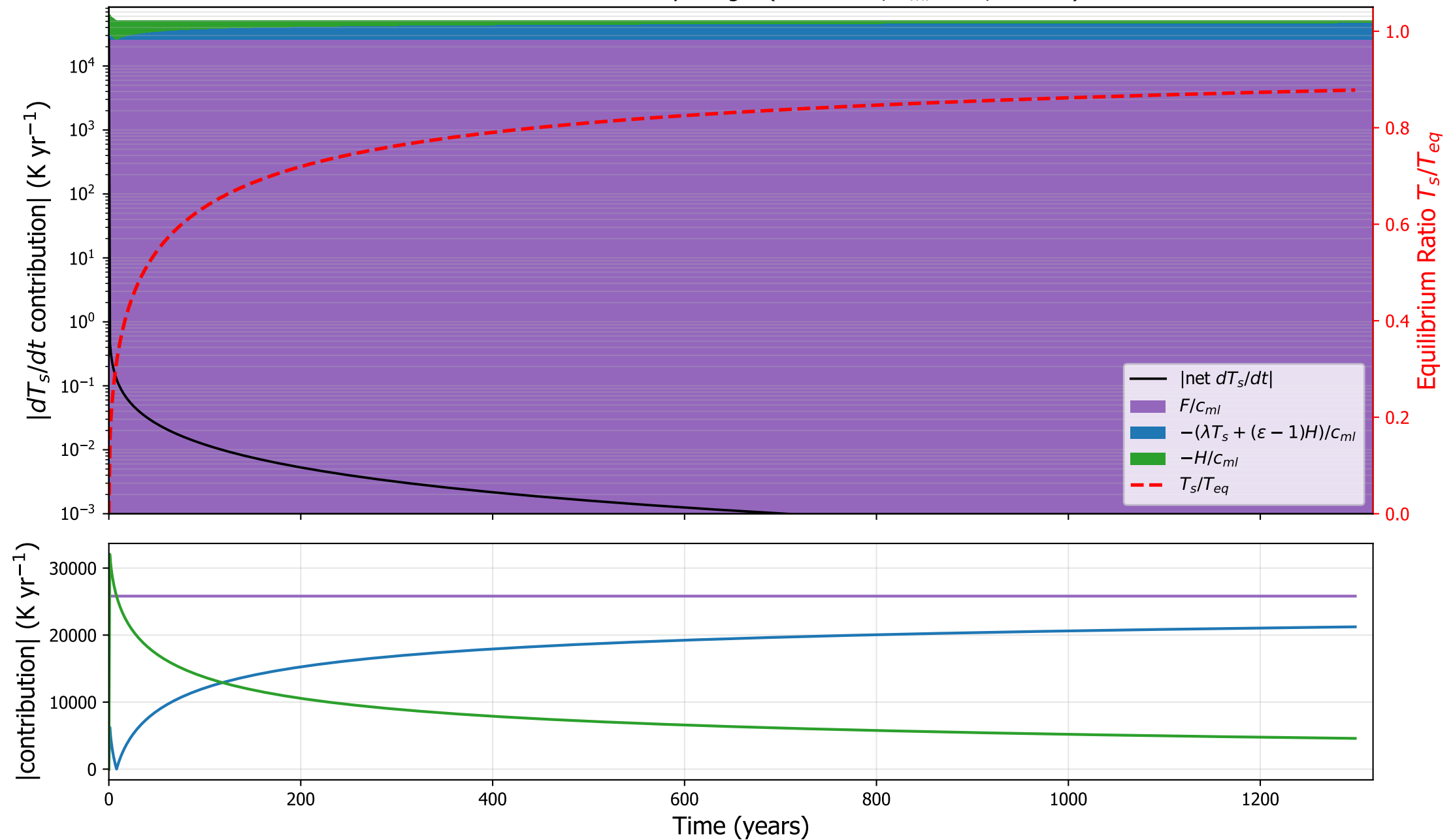
HadGEM2: surface tendency budget ( \kappa=4.0\text{e-}05 , h_{ml}=0 m, \varepsilon=0.69 )
