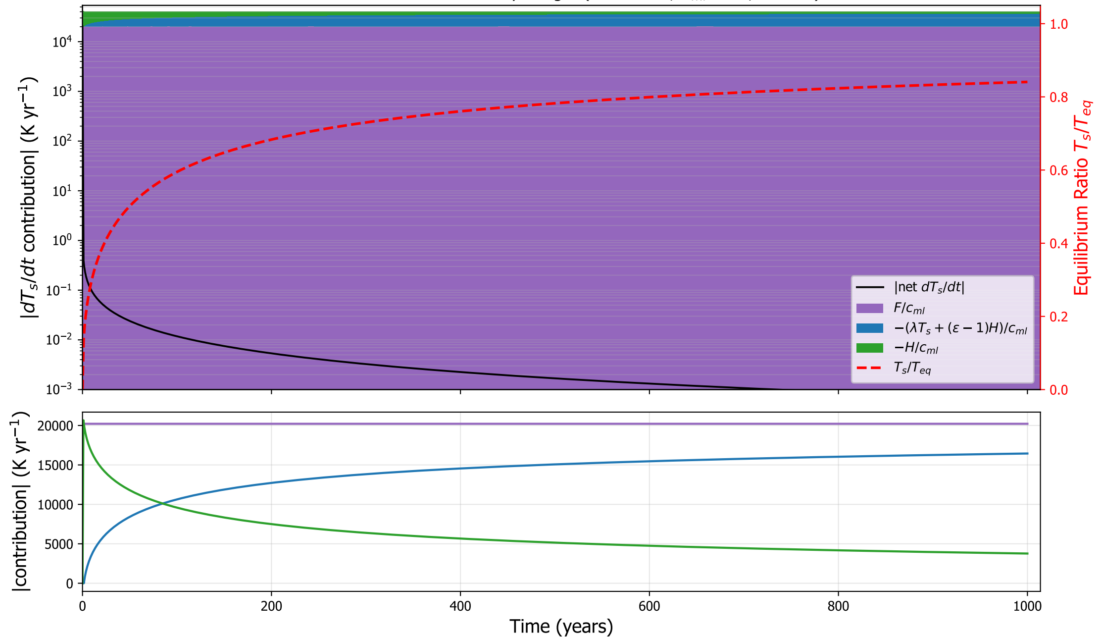
IPSLCM5A: surface tendency budget ( \kappa=5.2\text{e-}05 , h_{ml}=0 m, \varepsilon=0.85 )
