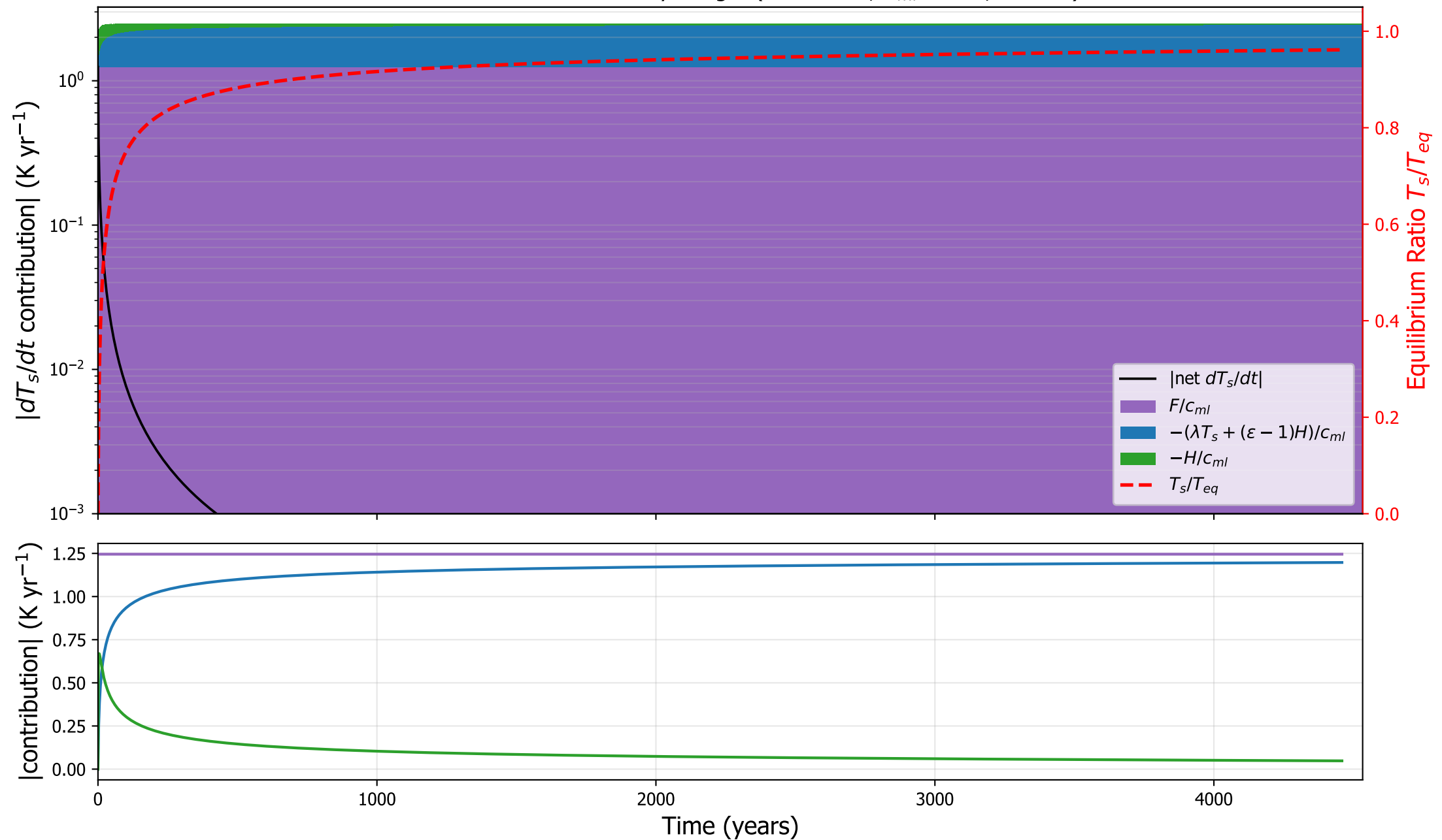
MPIESM11: surface tendency budget ( \kappa=2.9\text{e-}05 , h_{ml}=36 m, \varepsilon=1.00 )
