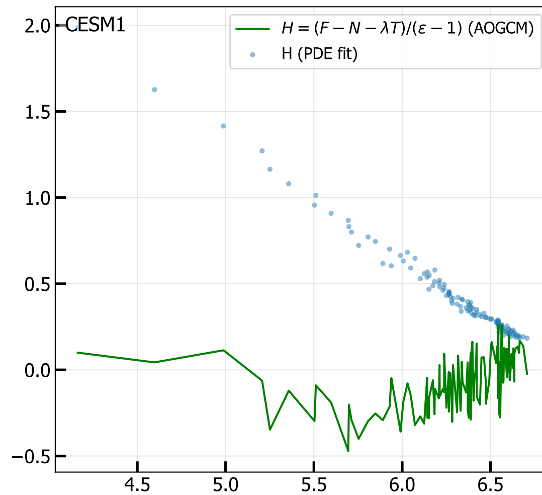
4xCO 2 Ocean Heat Uptake H vs T 2M
