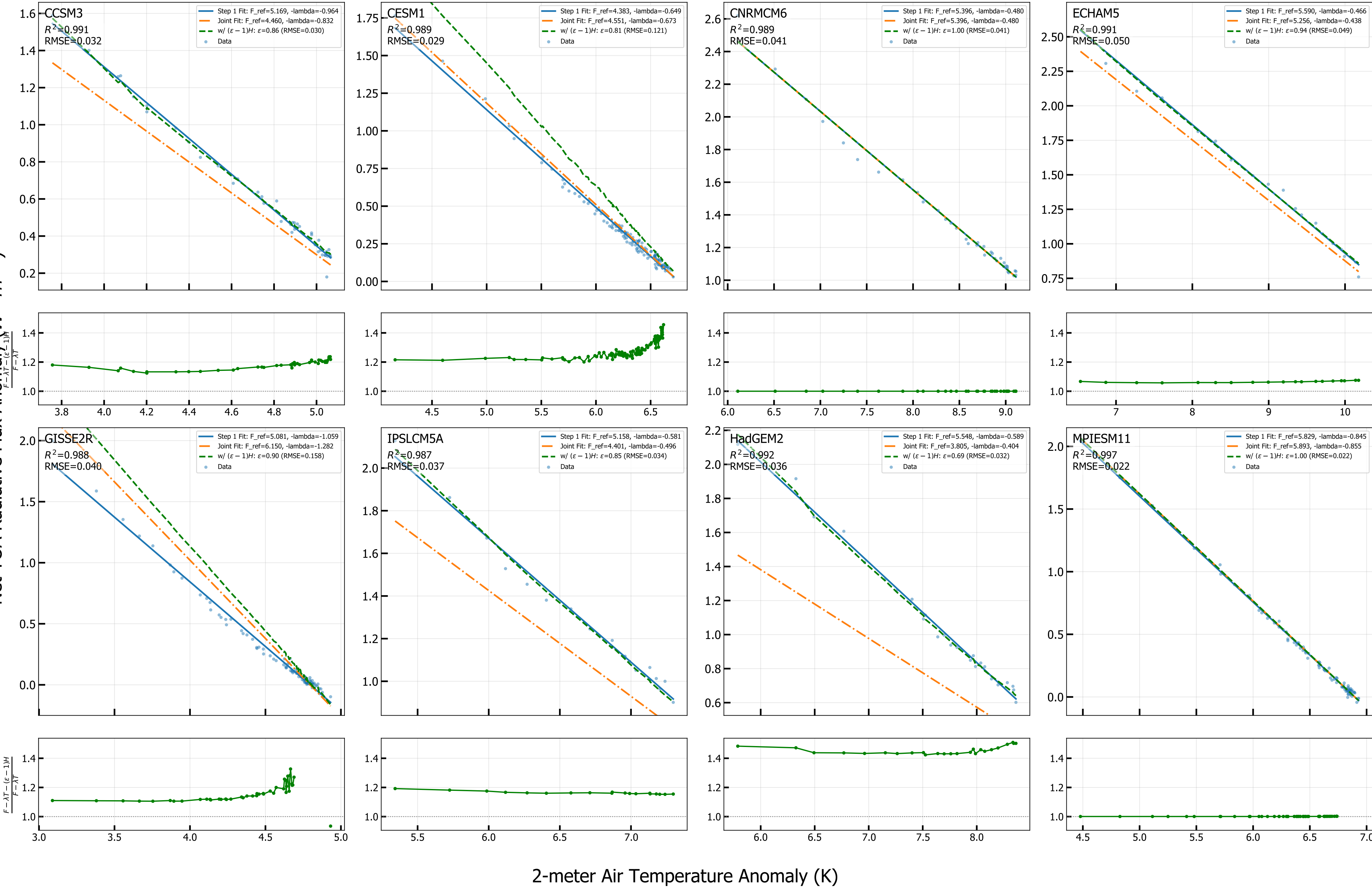
4xCO 2 Net TOA vs T 2M
