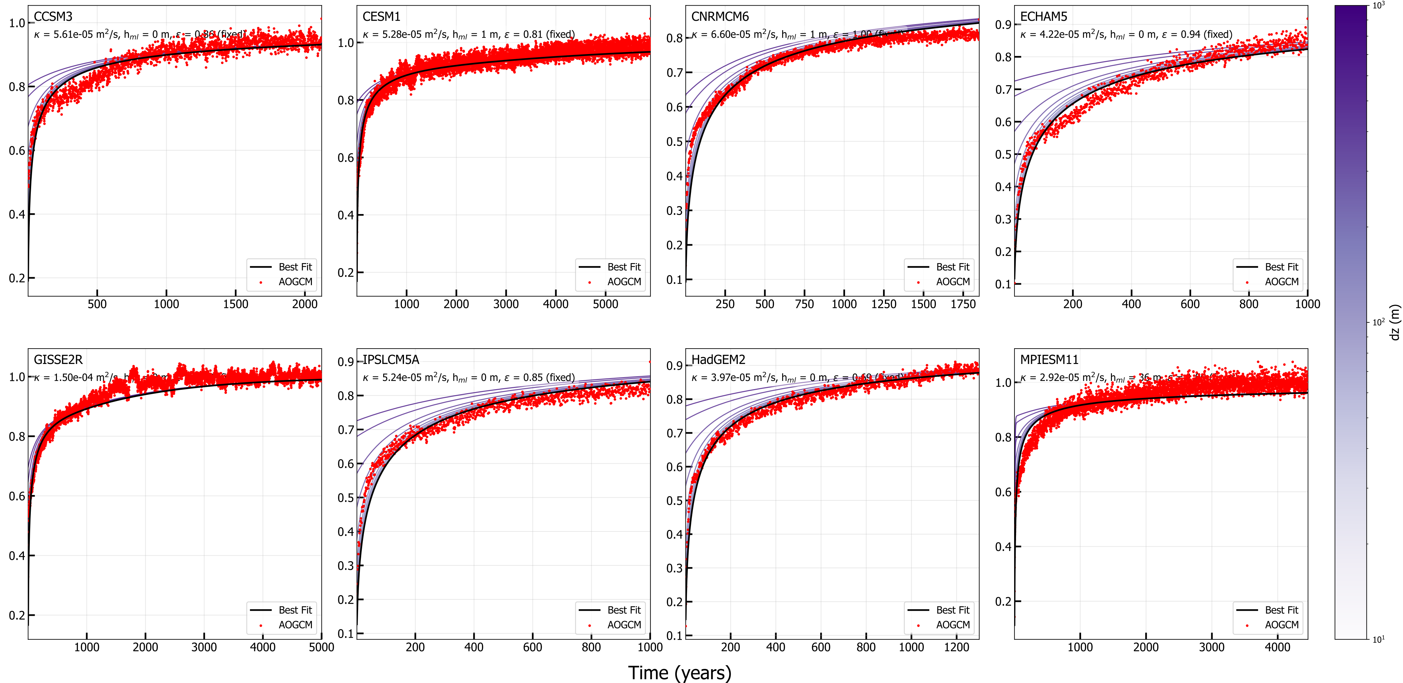
Sensitivity to Grid Spacing dz ( \kappa , h_{ml} held at best fit)
