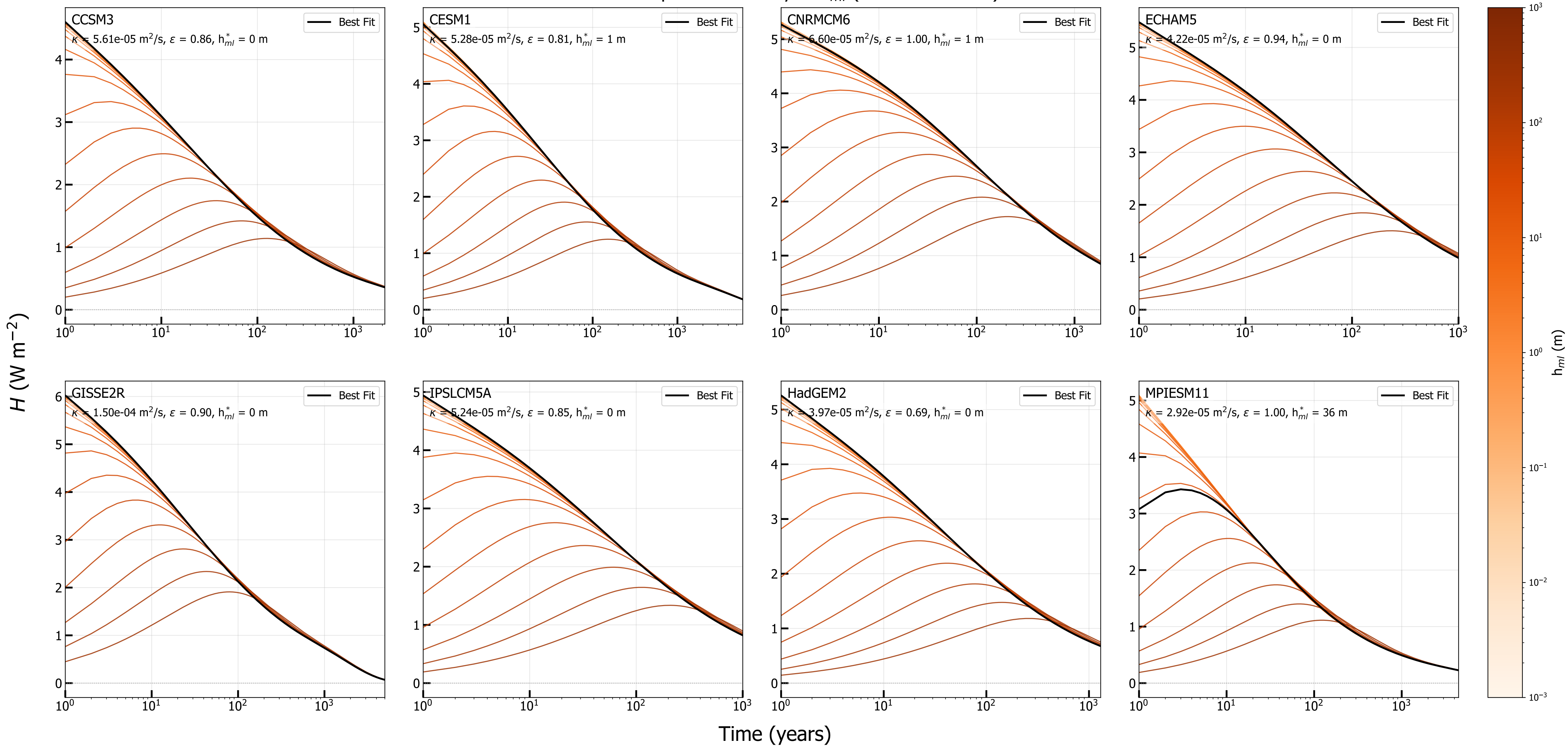
Ocean Heat Uptake Sensitivity to h_{ml} ( \kappa held at best fit)
