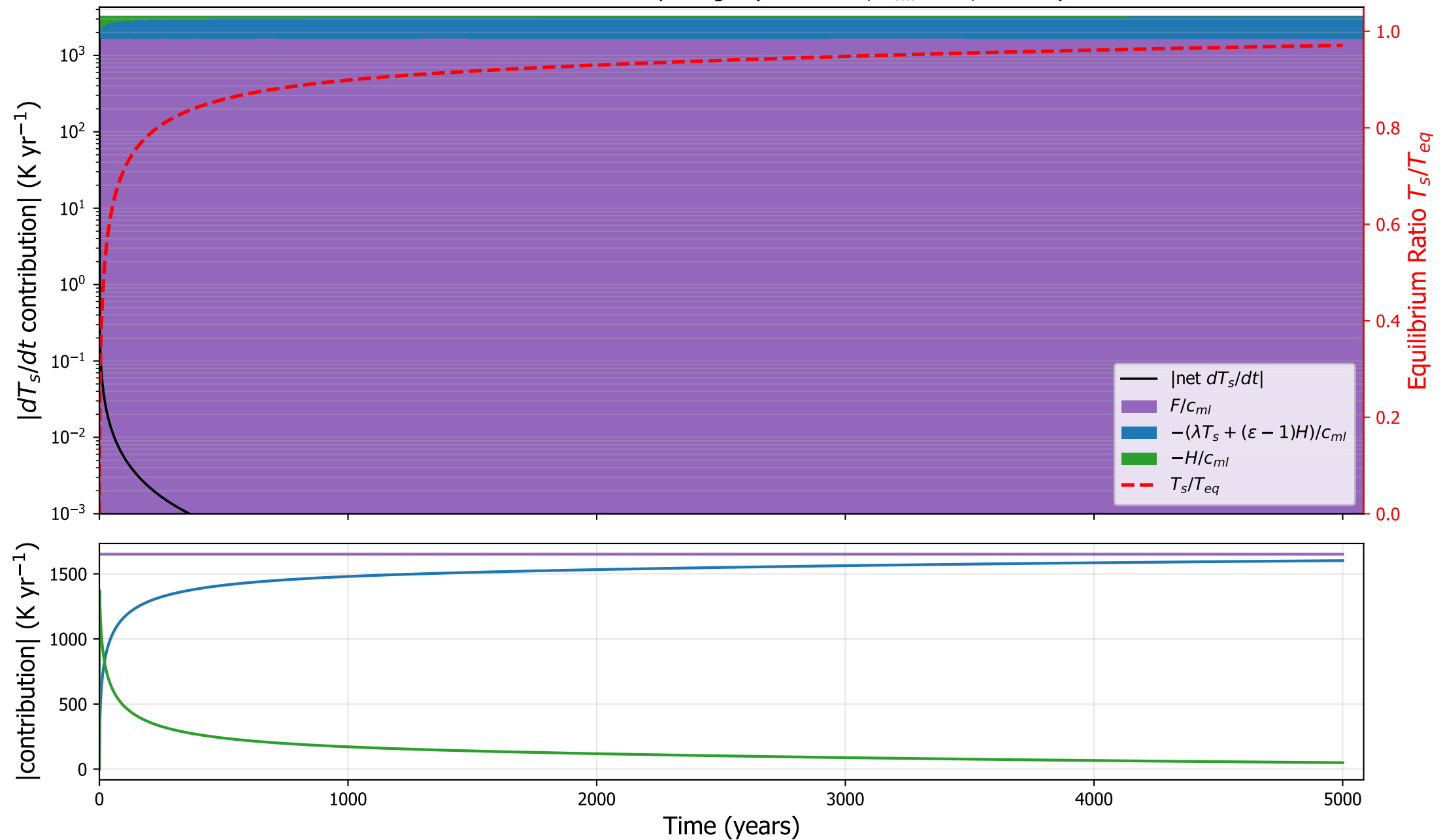
GISSE2R: surface tendency budget ( \kappa=6.7\text{e-}05 , h_{ml}=0 m, \varepsilon=0.98 )
