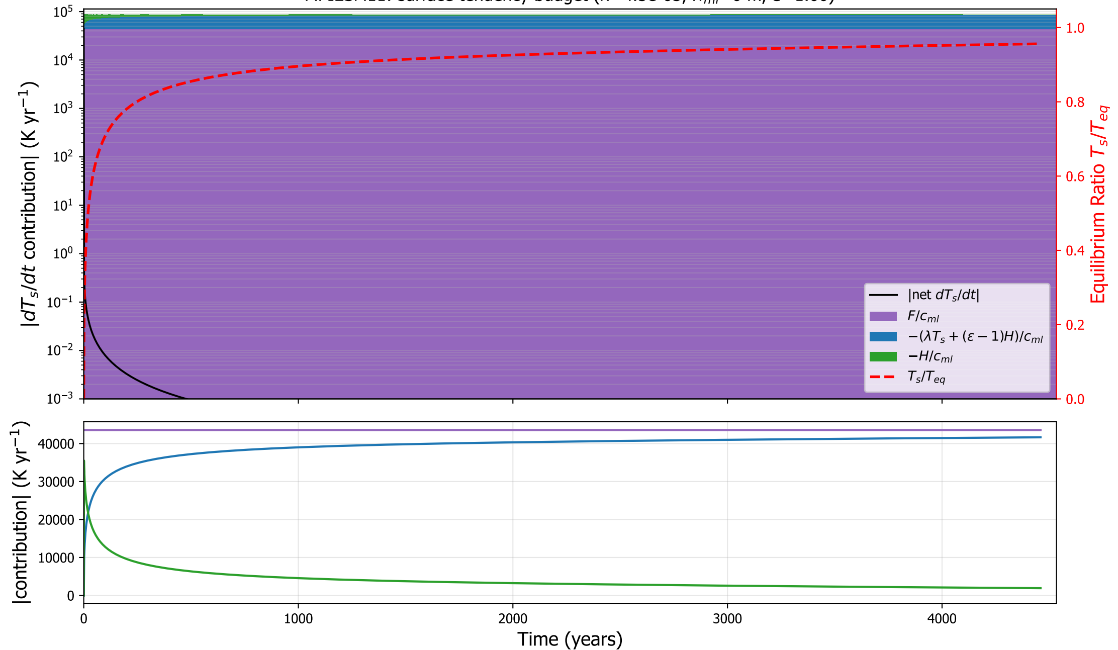
MPIESM11: surface tendency budget ( \kappa=4.5\text{e-}05 , h_{ml}=0 m, \varepsilon=1.00 )
