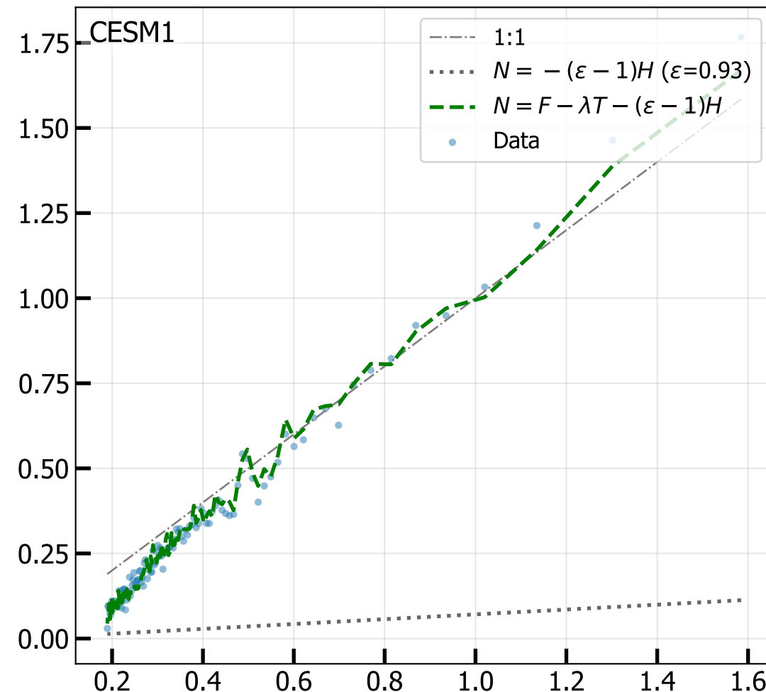
4xCO 2 Net TOA vs Ocean Heat Uptake H
