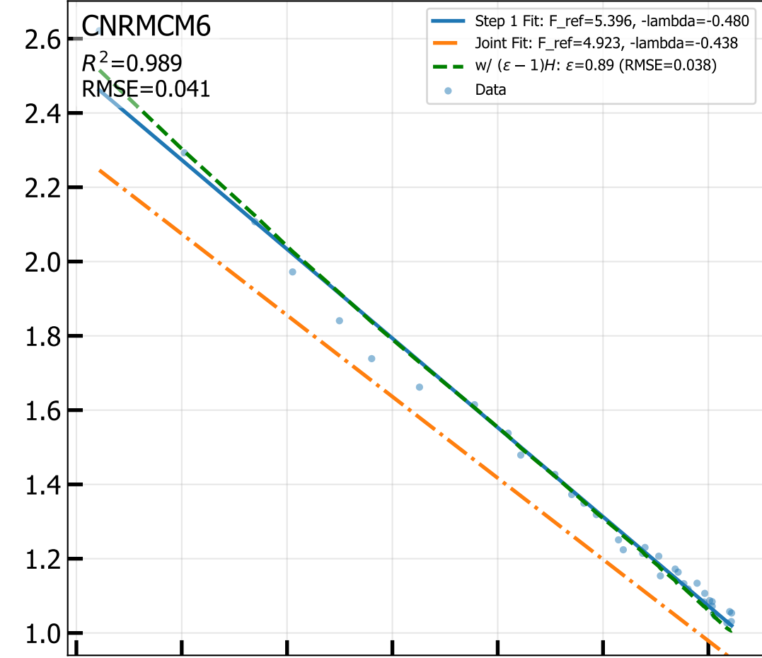
4xCO 2 Net TOA vs T 2M
