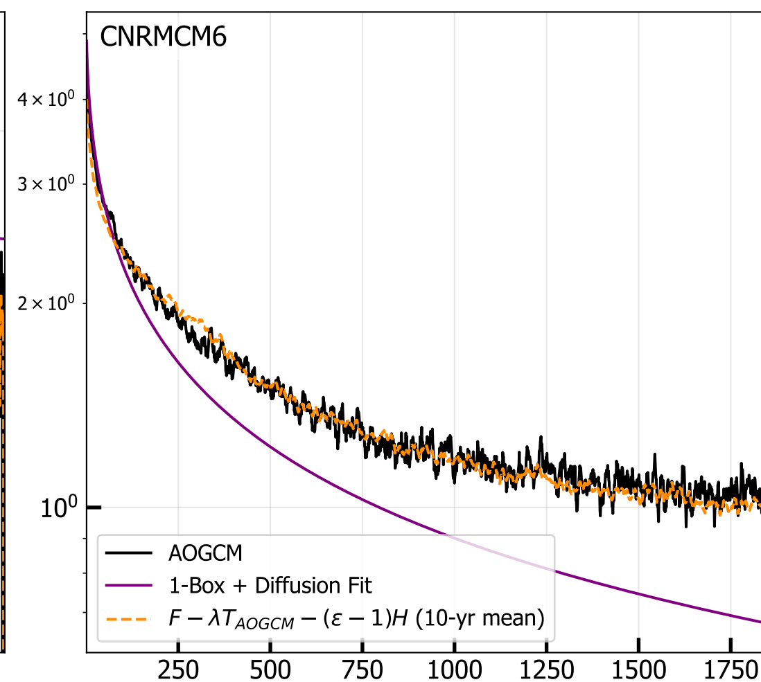
4xCO 2 Net TOA vs. Time
