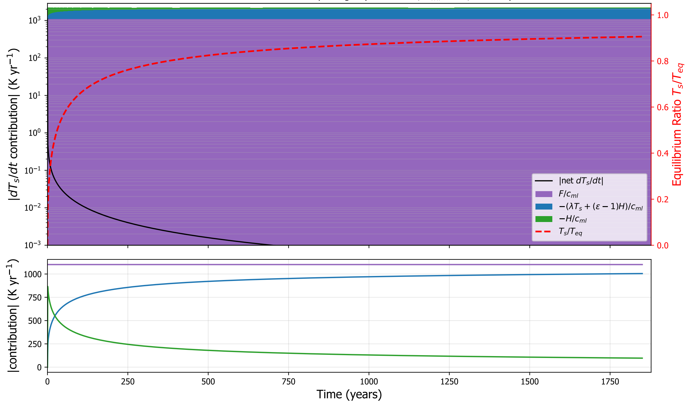
CNRMCM6: surface tendency budget ( \kappa=5.0\text{e-}05 , h_{ml}=0 m, \varepsilon=1.07 )
