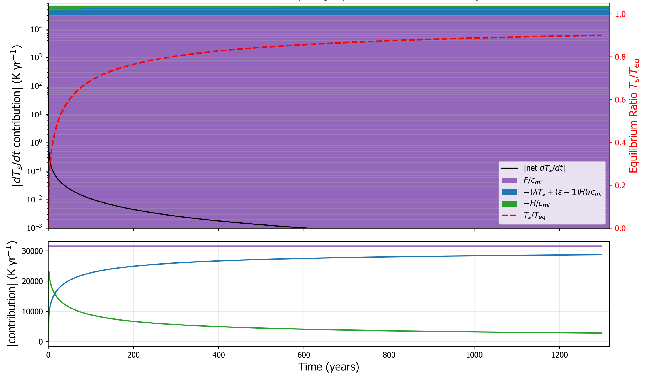
HadGEM2: surface tendency budget ( \kappa=3.3\text{e-}05 , h_{ml}=0 m, \varepsilon=1.11 )
