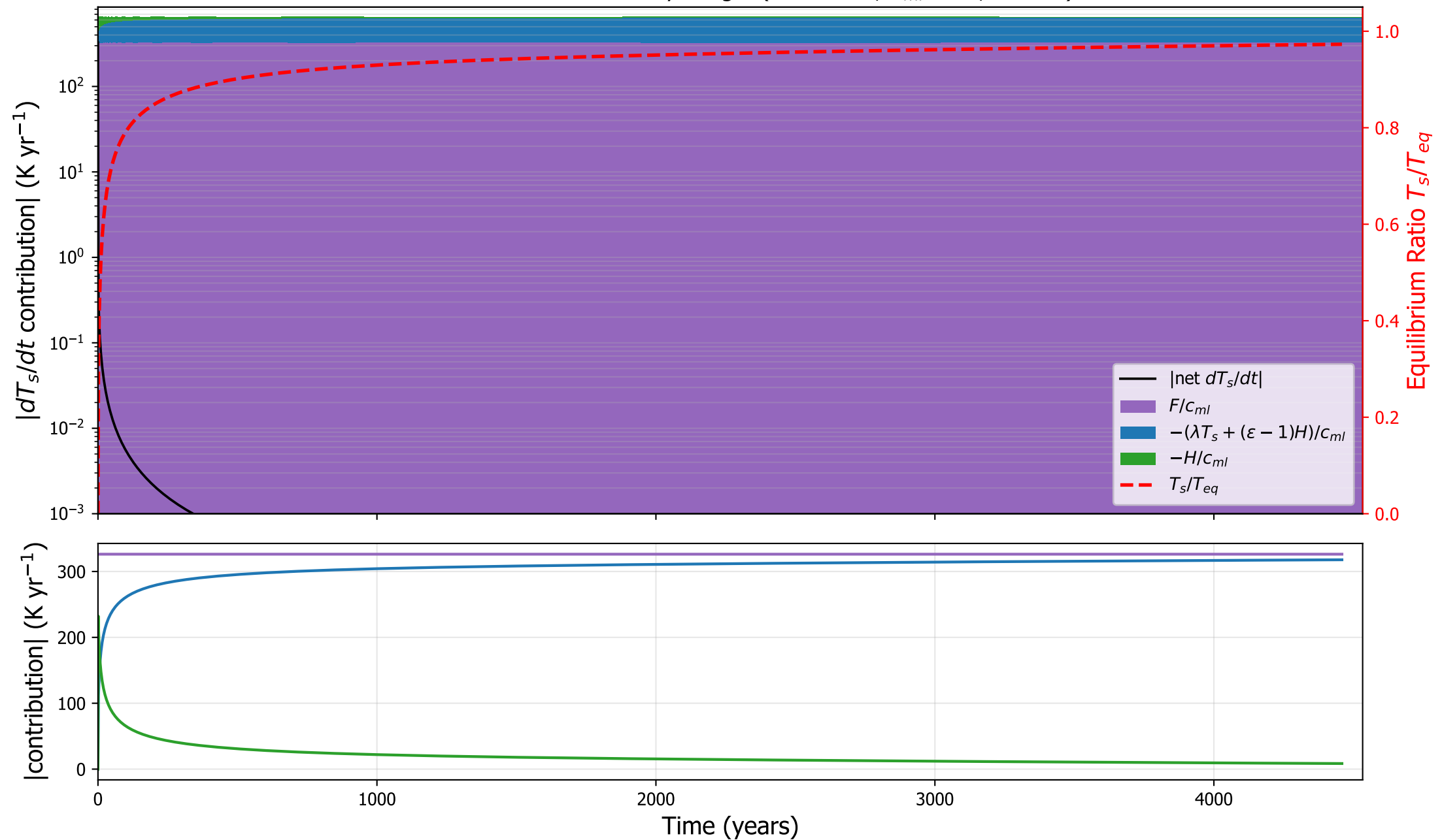
MPIESM11: surface tendency budget ( \kappa=5.2\text{e-}05 , h_{ml}=0 m, \varepsilon=1.04 )
