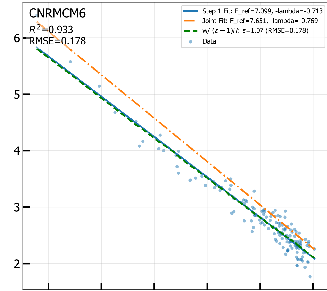
4xCO 2 Net TOA vs T 2M
