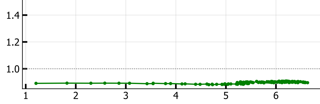
2-meter Air Temperature Anomaly (K)
