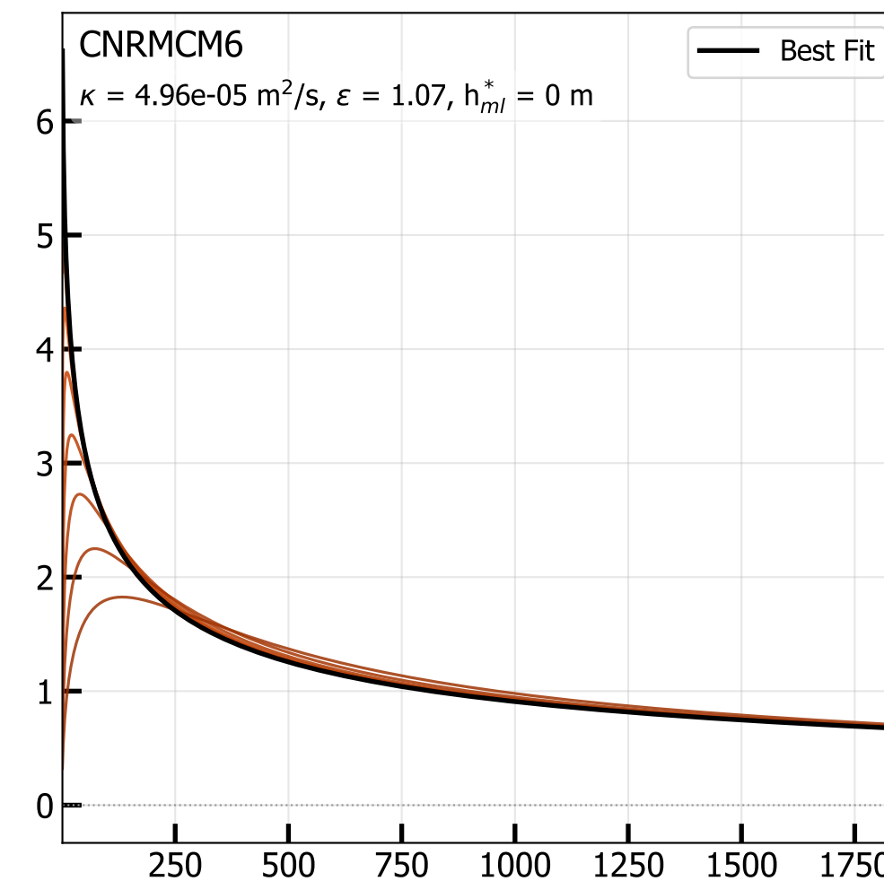
Ocean Heat Uptake Sensitivity to h_{ml} ( \kappa held at best fit)
