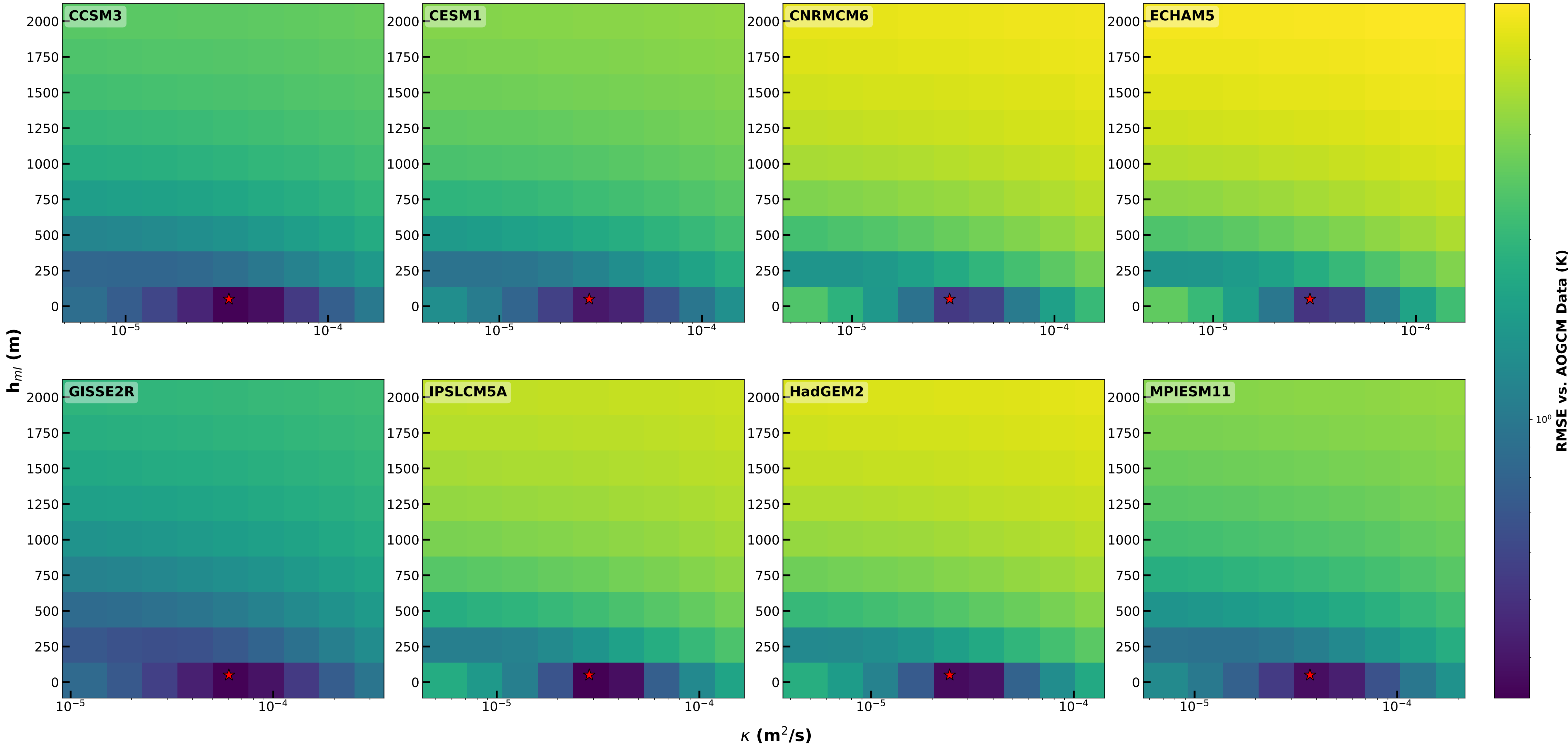
Fit RMSE vs. \kappa/h_{ml} (Parameter Degeneracy)
